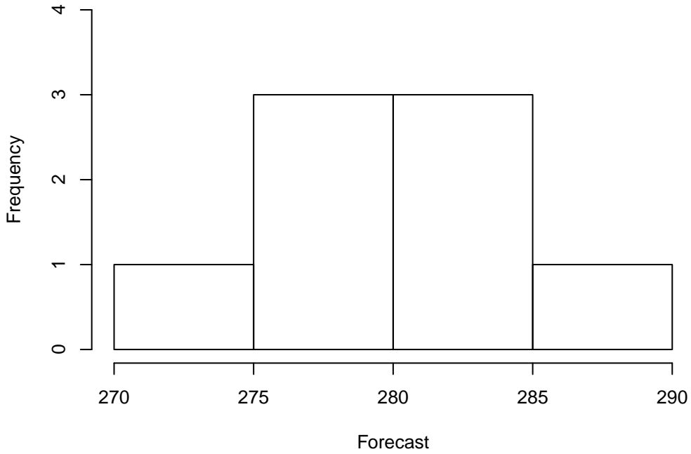
Forecast Histogram of 8 points WRF: TMP at P900-750 ADPSFC, DTC166, MEDIAN(9)
