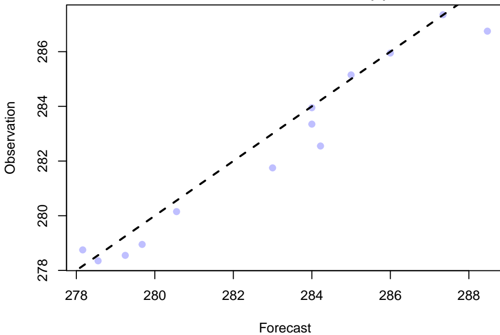
Scatter Plot of 13 points WRF: TMP at P900-750 ADPUPA, LMV, MEDIAN(9)
