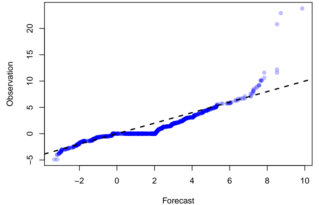
Q-Q Plot of 934 points WRF: UGRD at Z10 ADPSFC, DTC165, DW_MEAN(9)
