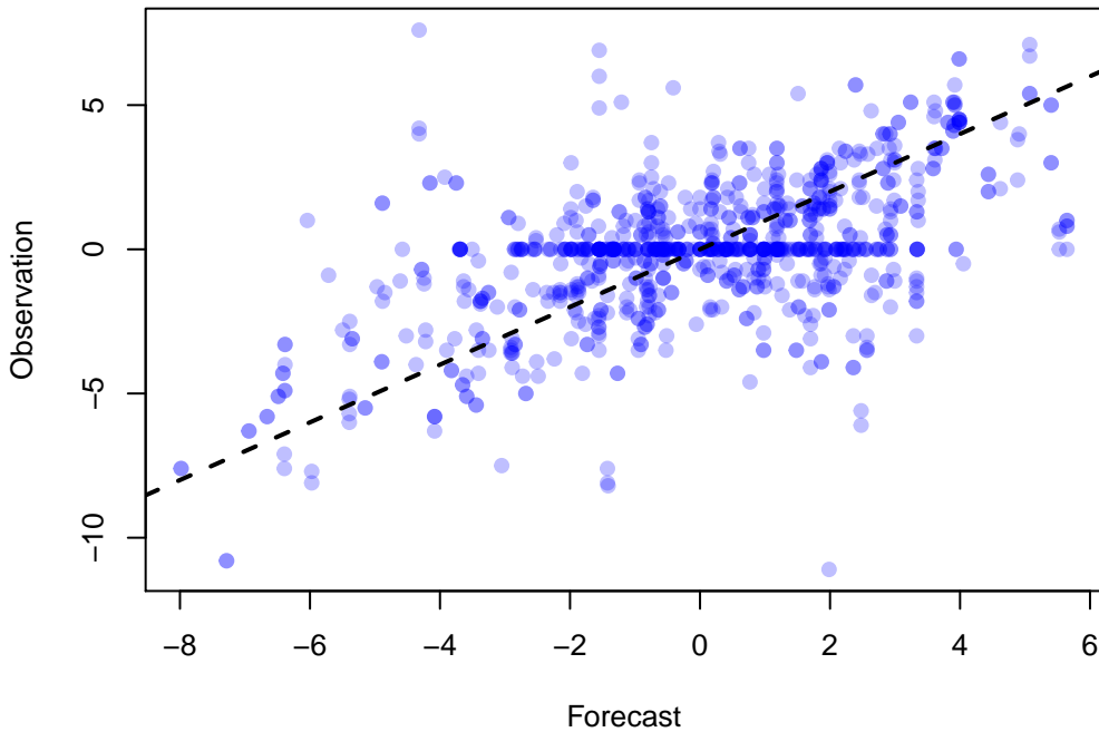
Scatter Plot of 934 points WRF: VGRD at Z10 ADPSFC, DTC165, MEDIAN(9)
