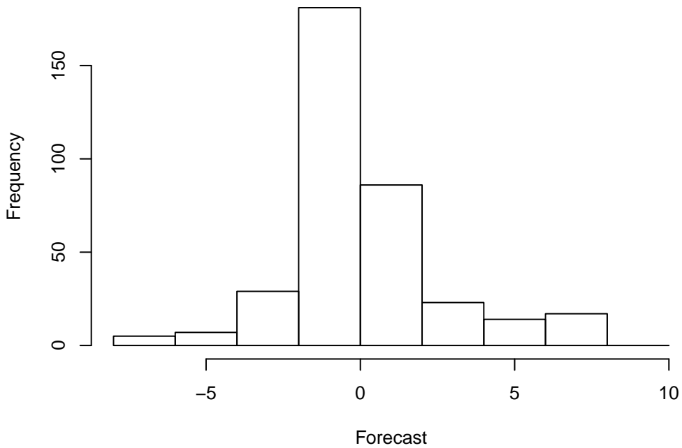
Forecast Histogram of 362 points WRF: UGRD at Z10 ADPSFC, LMV, DW_MEAN(9)
