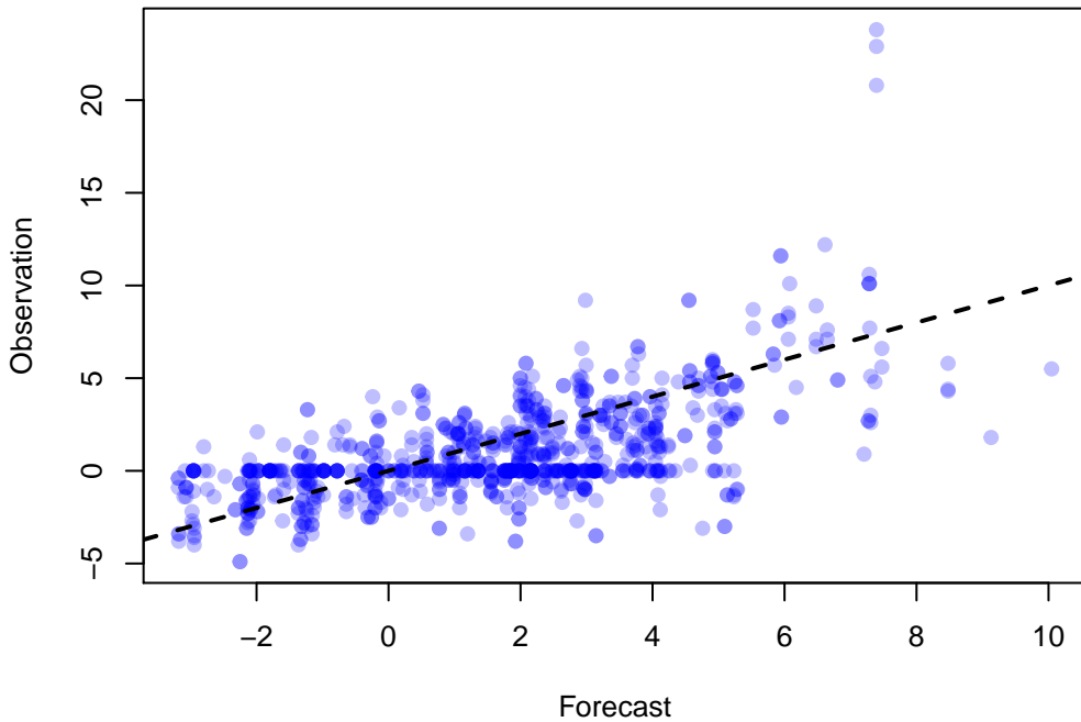
Scatter Plot of 934 points WRF: UGRD at Z10 ADPSFC, DTC165, MEDIAN(9)
