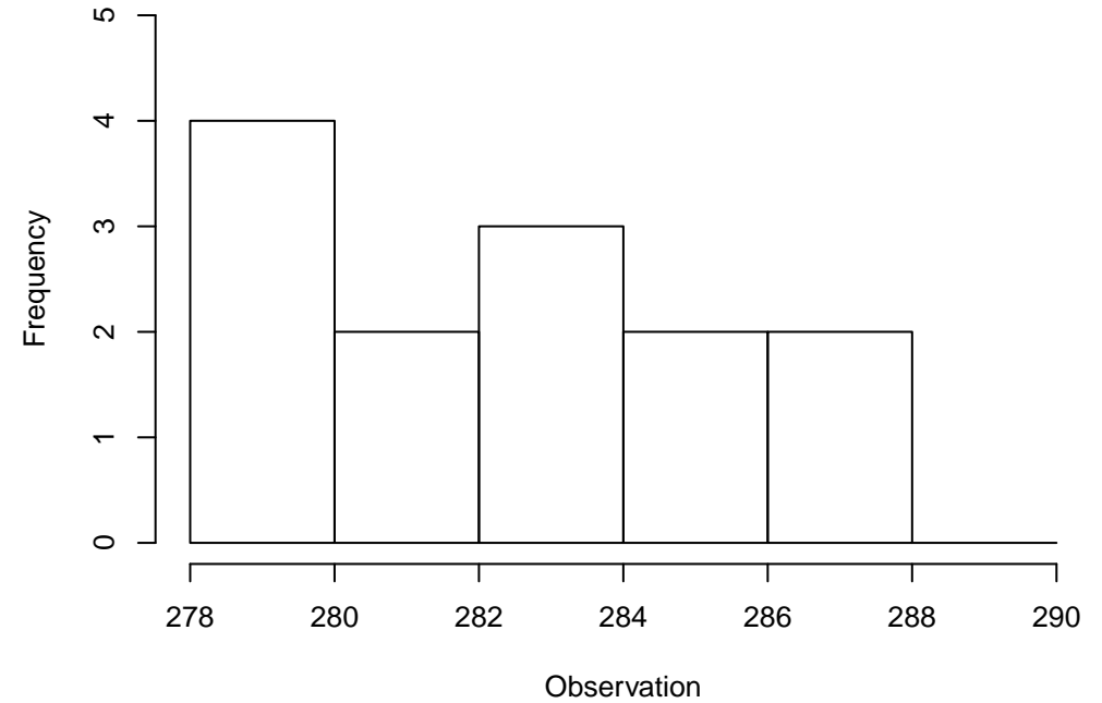
Observation Histogram of 13 points WRF: TMP at P900-750 ADPUPA, LMV, UW_MEAN(1)
