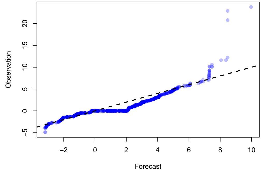
Q-Q Plot of 934 points WRF: UGRD at Z10 ADPSFC, DTC165, UW_MEAN(1)
