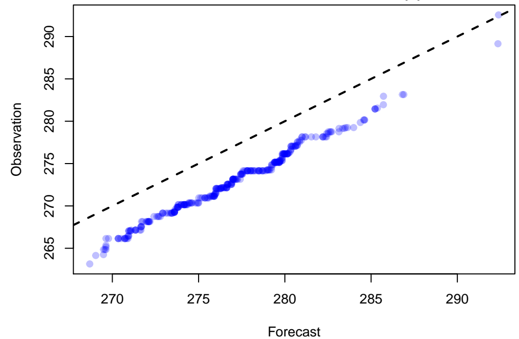
Q-Q Plot of 326 points WRF: TMP at P900-750 ADPSFC, DTC165, UW_MEAN(1)
