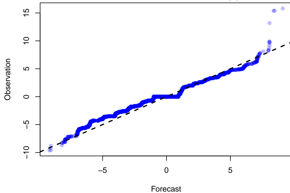
Q-Q Plot of 2955 points WRF: UGRD at Z10 ADPSFC, DTC166, DW_MEAN(9)
