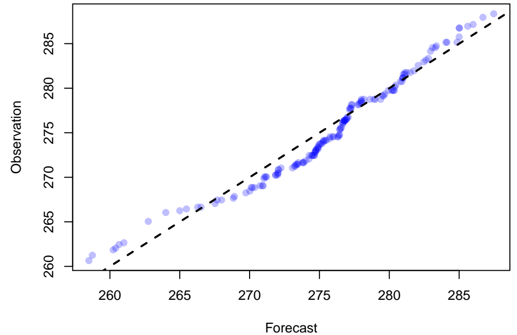
Q-Q Plot of 155 points WRF: TMP at P900-750 ADPUPA, DTC165, DW_MEAN(9)
