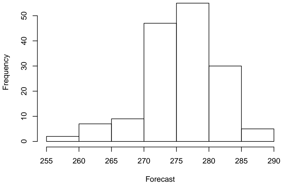
Forecast Histogram of 155 points WRF: TMP at P900-750 ADPUPA, DTC165, DW_MEAN(9)
