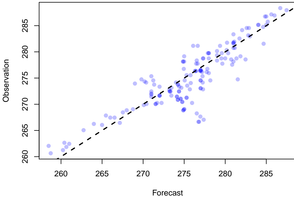
Scatter Plot of 155 points WRF: TMP at P900-750 ADPUPA, DTC165, MEDIAN(9)
