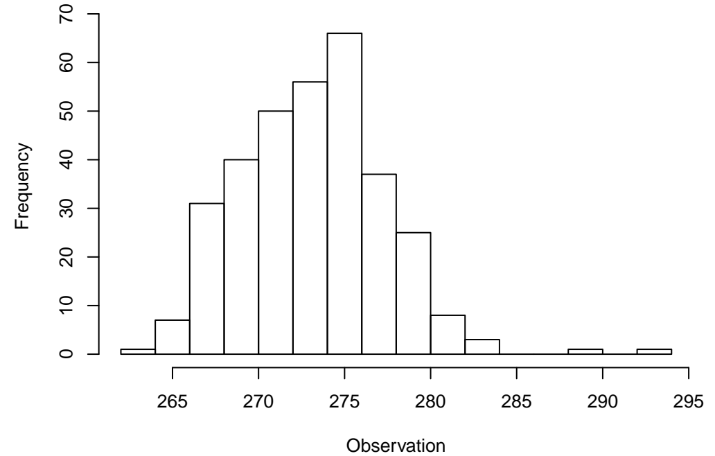
Observation Histogram of 326 points WRF: TMP at P900-750 ADPSFC, DTC165, MEDIAN(9)
