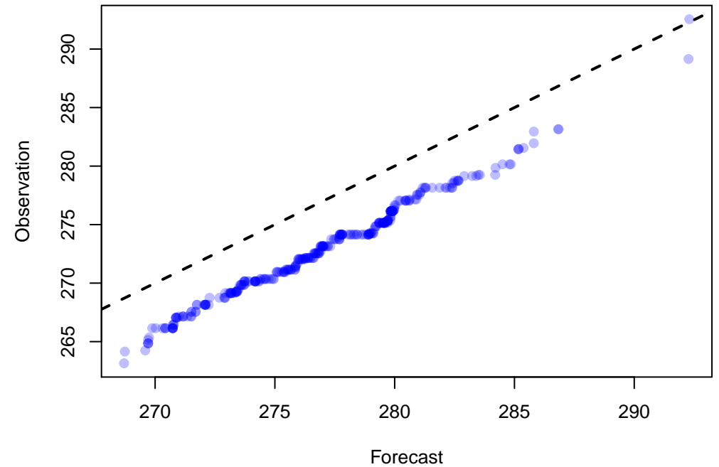
Q-Q Plot of 326 points WRF: TMP at P900-750 ADPSFC, DTC165, DW_MEAN(9)
