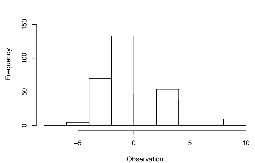
Observation Histogram of 362 points WRF: UGRD at Z10 ADPSFC, LMV, MEDIAN(9)
