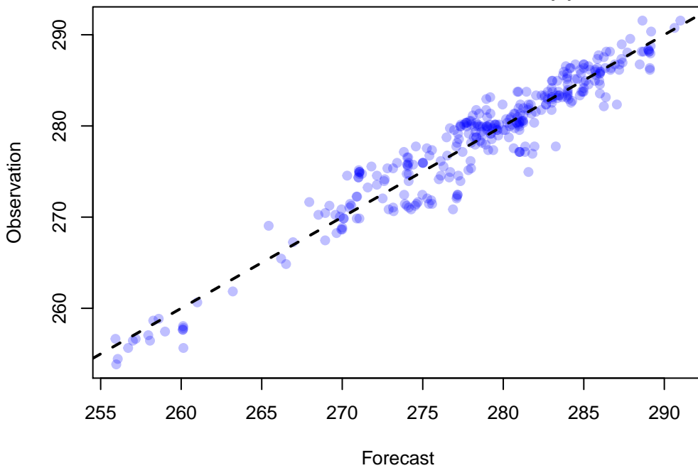
Scatter Plot of 334 points WRF: TMP at P900-750 ADPUPA, DTC166, DW_MEAN(9)
