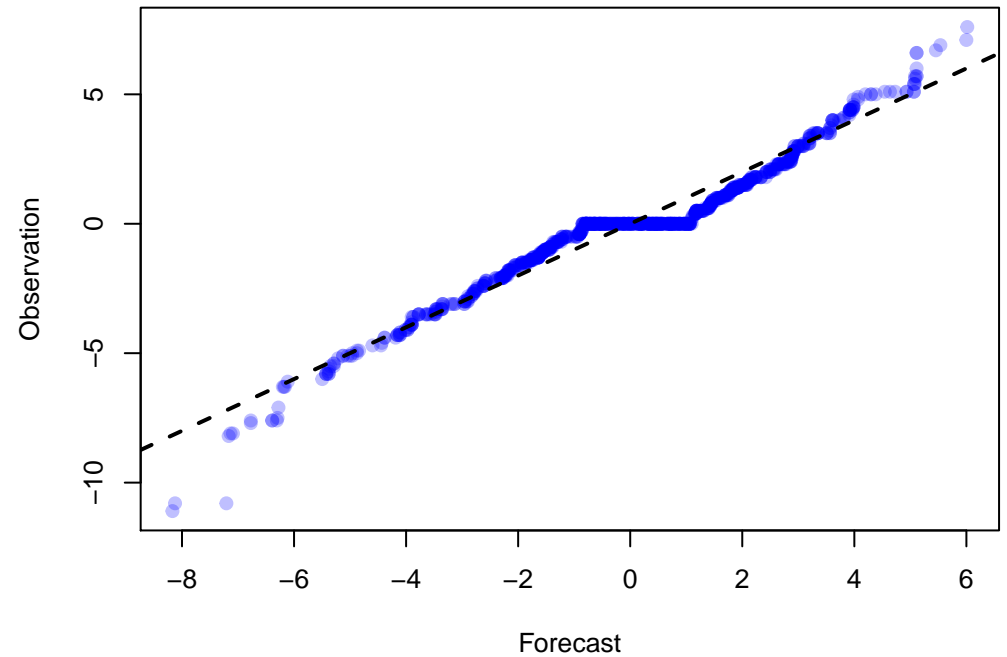
Q-Q Plot of 934 points WRF: VGRD at Z10 ADPSFC, DTC165, DW_MEAN(9)
