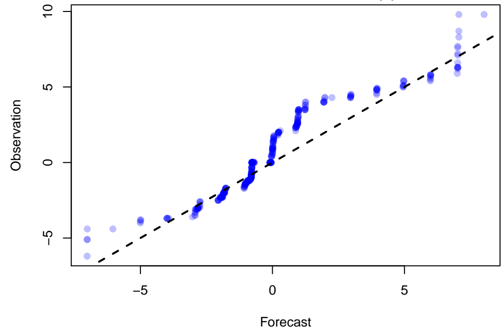
Q-Q Plot of 362 points WRF: UGRD at Z10 ADPSFC, LMV, UW_MEAN(1)
