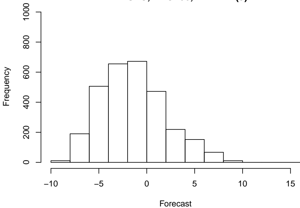
Forecast Histogram of 2955 points WRF: UGRD at Z10 ADPSFC, DTC166, MEDIAN(9)
