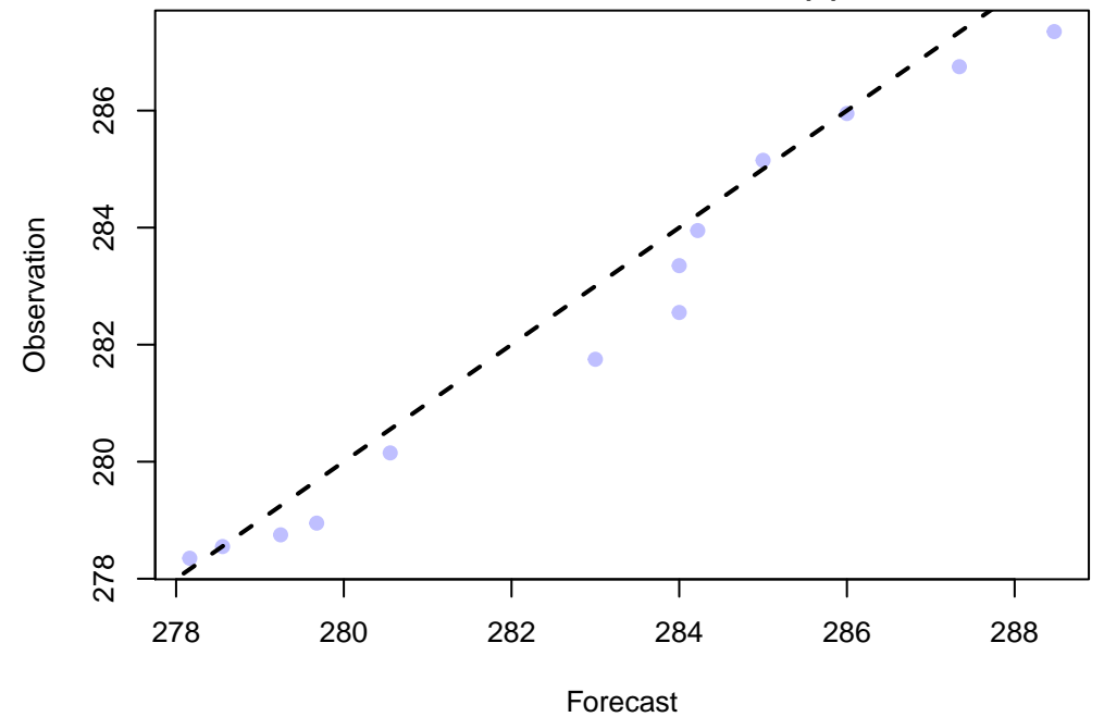
Q-Q Plot of 13 points WRF: TMP at P900-750 ADPUPA, LMV, MEDIAN(9)
