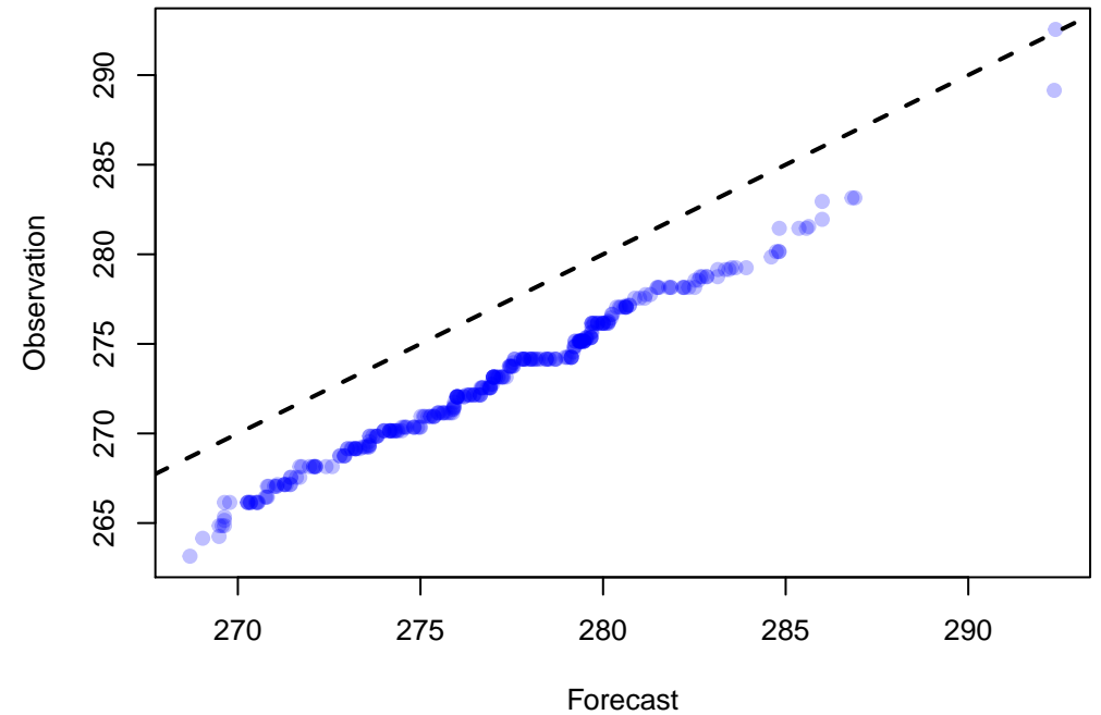
Q-Q Plot of 326 points WRF: TMP at P900-750 ADPSFC, DTC165, MEDIAN(9)
