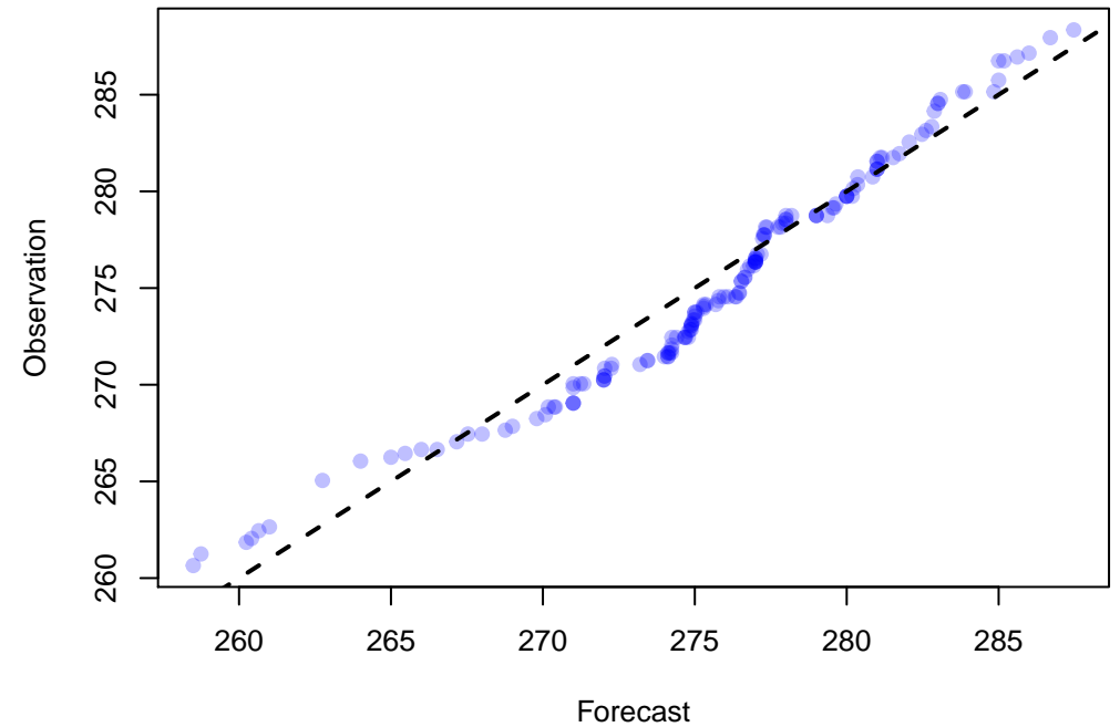
Q-Q Plot of 155 points WRF: TMP at P900-750 ADPUPA, DTC165, UW_MEAN(1)
