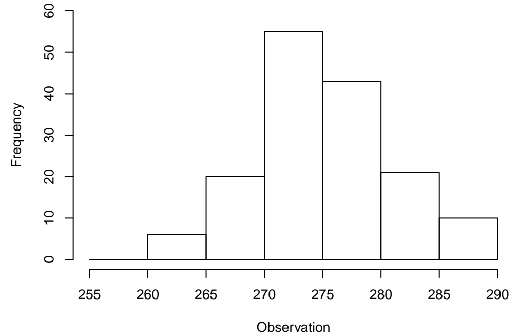
Observation Histogram of 155 points WRF: TMP at P900-750 ADPUPA, DTC165, UW_MEAN(1)
