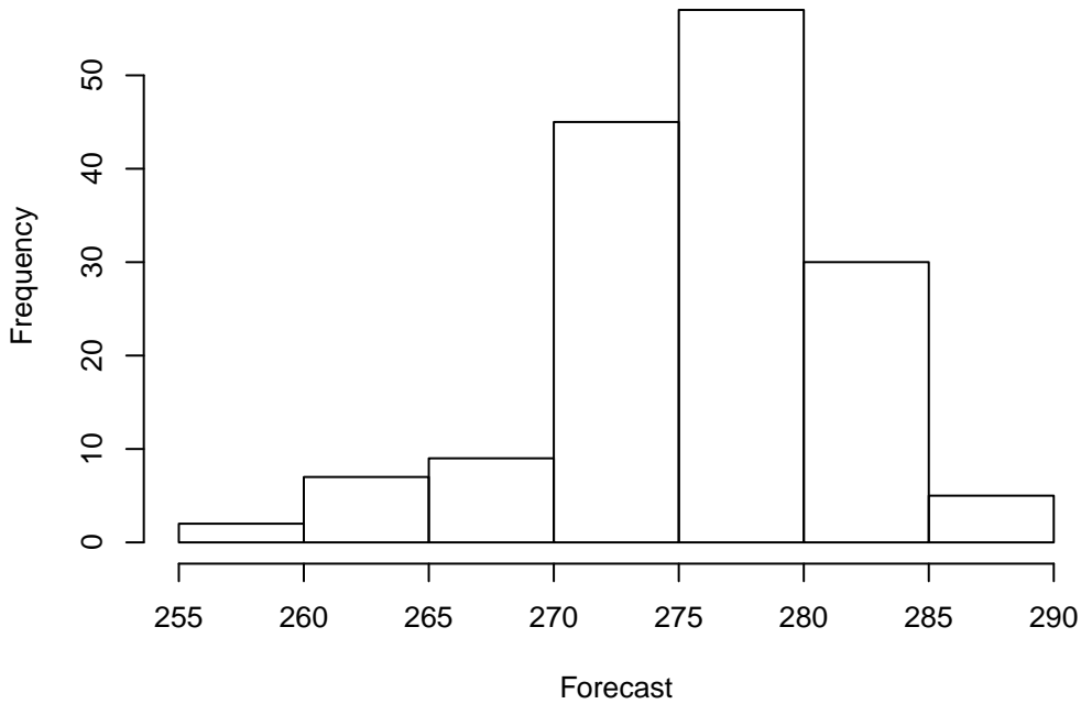
Forecast Histogram of 155 points WRF: TMP at P900-750 ADPUPA, DTC165, MEDIAN(9)
