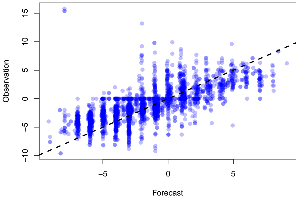
Scatter Plot of 2955 points WRF: UGRD at Z10 ADPSFC, DTC166, MEDIAN(9)
