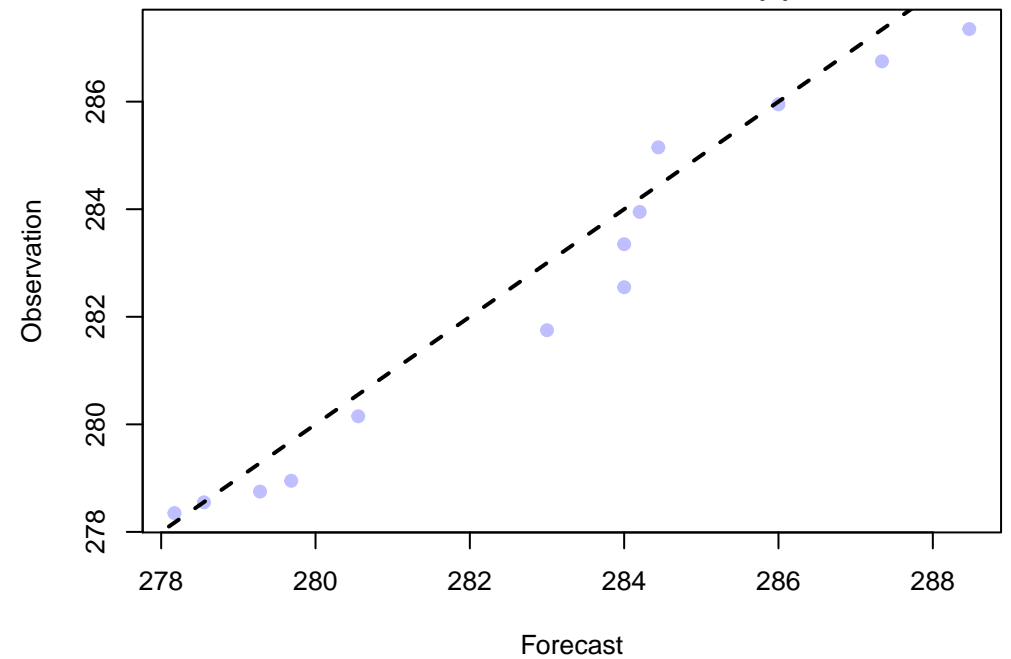
Q-Q Plot of 13 points WRF: TMP at P900-750 ADPUPA, LMV, DW_MEAN(9)
