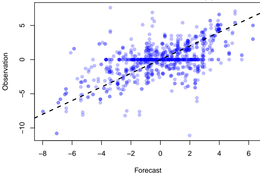
Scatter Plot of 934 points WRF: VGRD at Z10 ADPSFC, DTC165, UW_MEAN(1)
