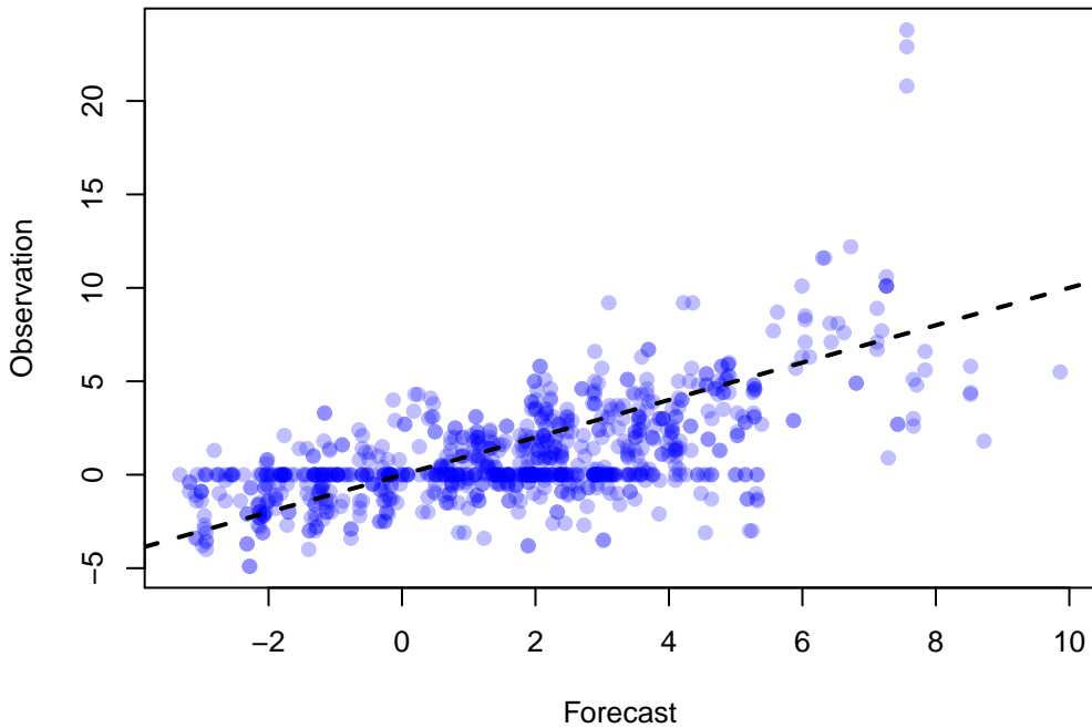
Scatter Plot of 934 points WRF: UGRD at Z10 ADPSFC, DTC165, DW_MEAN(9)
