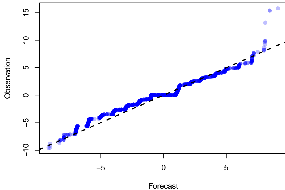
Q-Q Plot of 2955 points WRF: UGRD at Z10 ADPSFC, DTC166, MEDIAN(9)
