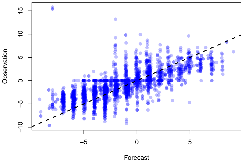
Scatter Plot of 2955 points WRF: UGRD at Z10 ADPSFC, DTC166, UW_MEAN(1)
