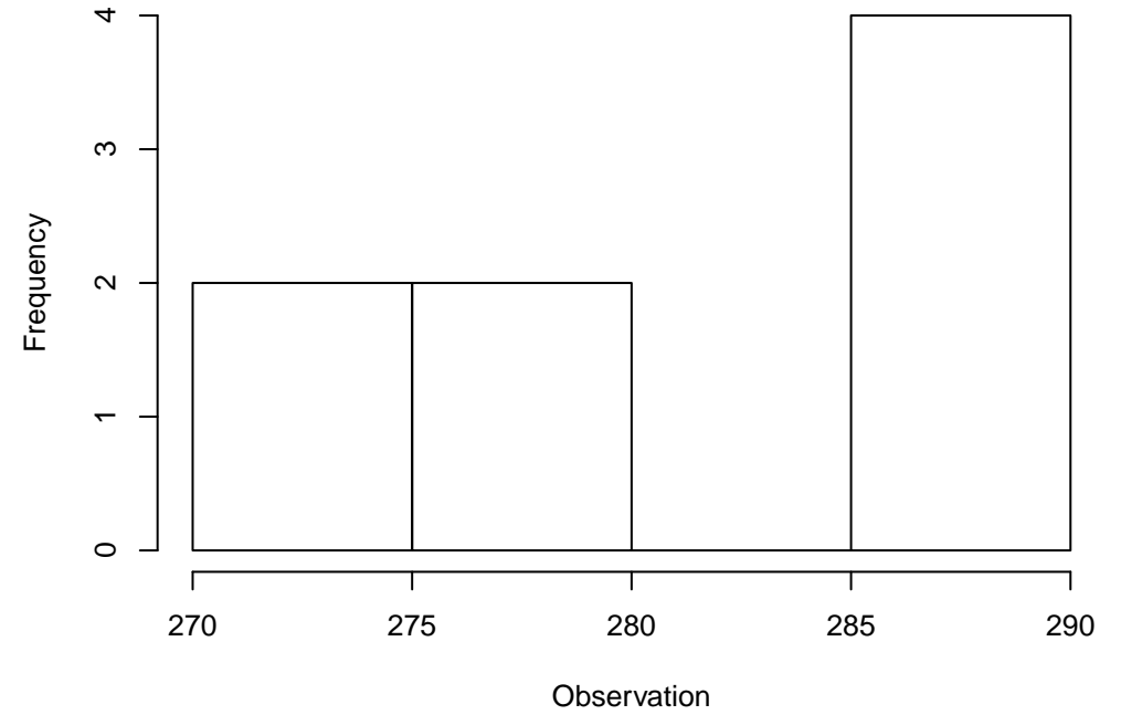
Observation Histogram of 8 points WRF: TMP at P900-750 ADPSFC, DTC166, DW_MEAN(9)
