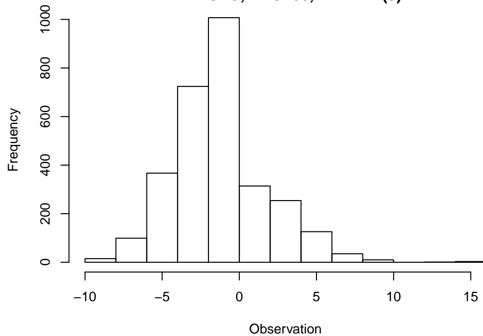
Observation Histogram of 2955 points WRF: UGRD at Z10 ADPSFC, DTC166, MEDIAN(9)
