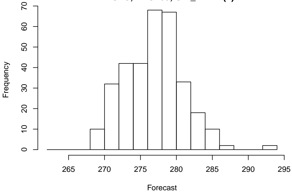
Forecast Histogram of 326 points WRF: TMP at P900-750 ADPSFC, DTC165, UW_MEAN(1)
