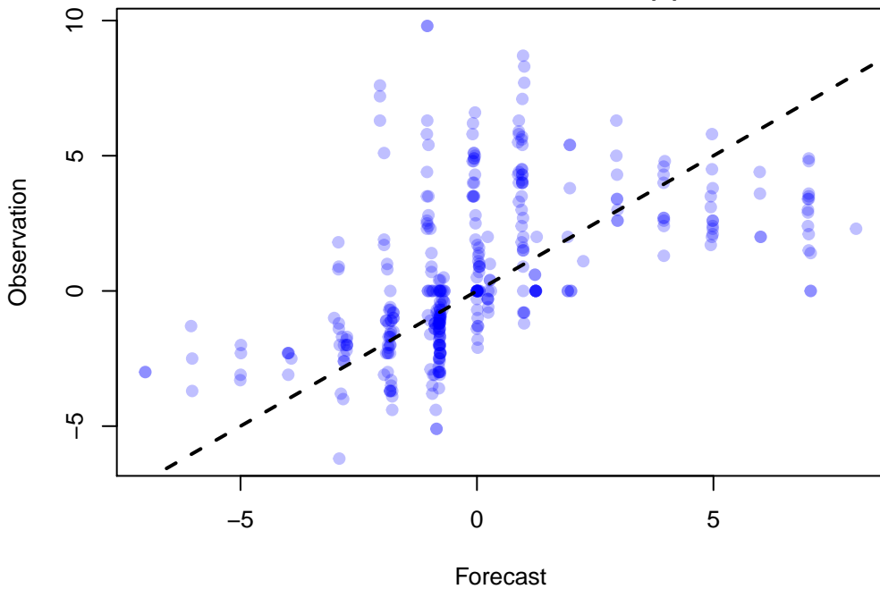
Scatter Plot of 362 points WRF: UGRD at Z10 ADPSFC, LMV, MEDIAN(9)
