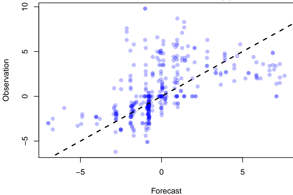
Scatter Plot of 362 points WRF: UGRD at Z10 ADPSFC, LMV, DW_MEAN(9)
