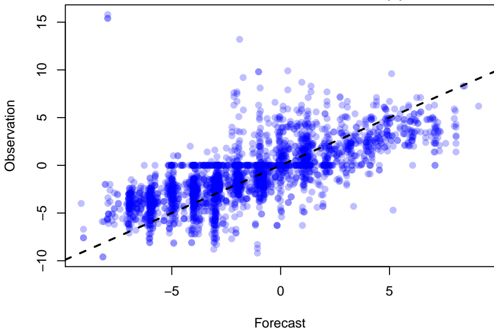
Scatter Plot of 2955 points WRF: UGRD at Z10 ADPSFC, DTC166, DW_MEAN(9)
