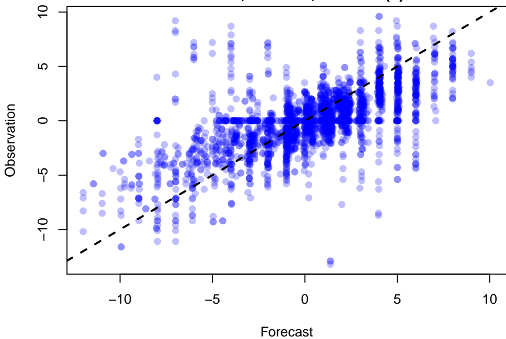
Scatter Plot of 2955 points WRF: VGRD at Z10 ADPSFC, DTC166, MEDIAN(9)
