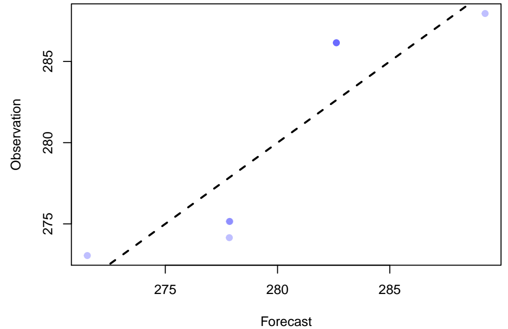
Q-Q Plot of 8 points WRF: TMP at P900-750 ADPSFC, DTC166, UW_MEAN(1)
