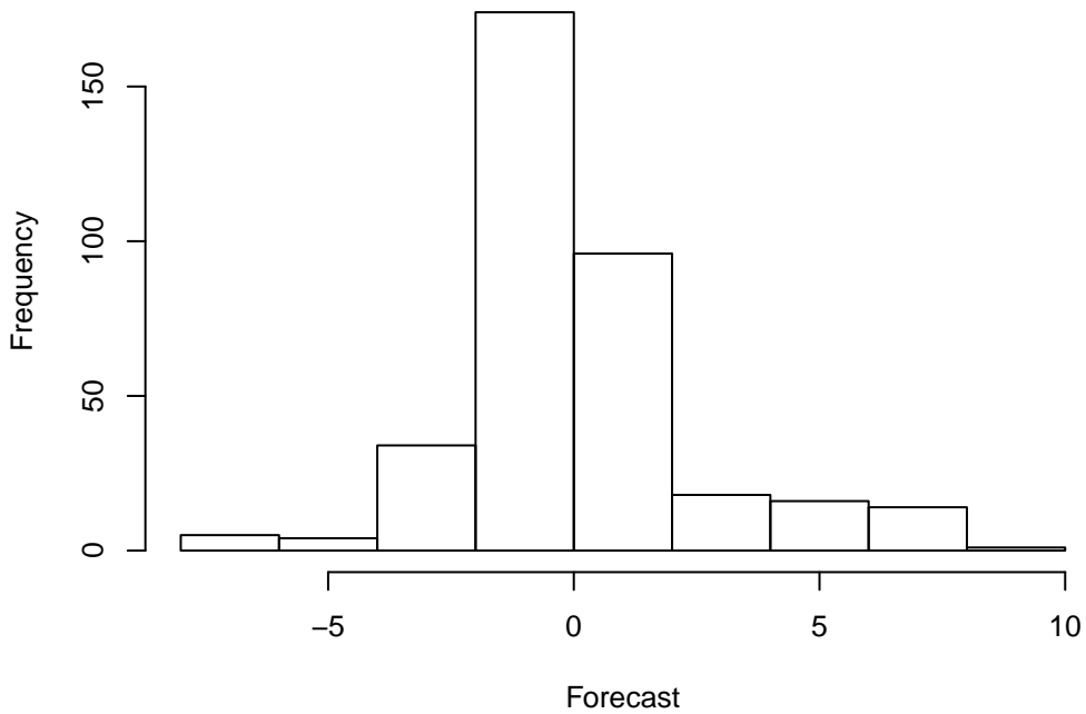
Forecast Histogram of 362 points WRF: UGRD at Z10 ADPSFC, LMV, UW_MEAN(1)
