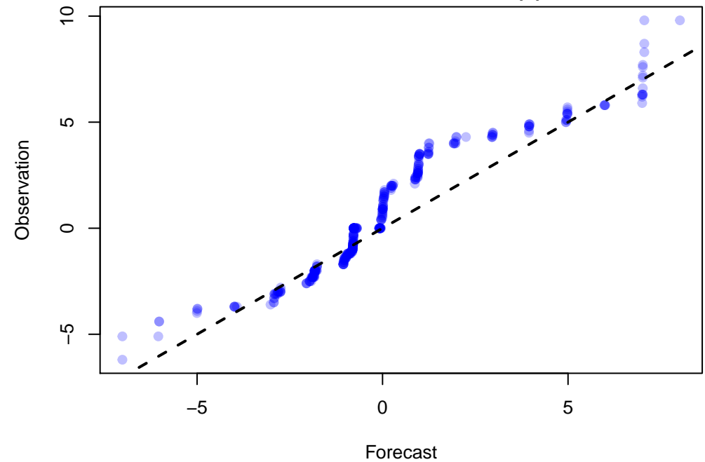
Q-Q Plot of 362 points WRF: UGRD at Z10 ADPSFC, LMV, MEDIAN(9)
