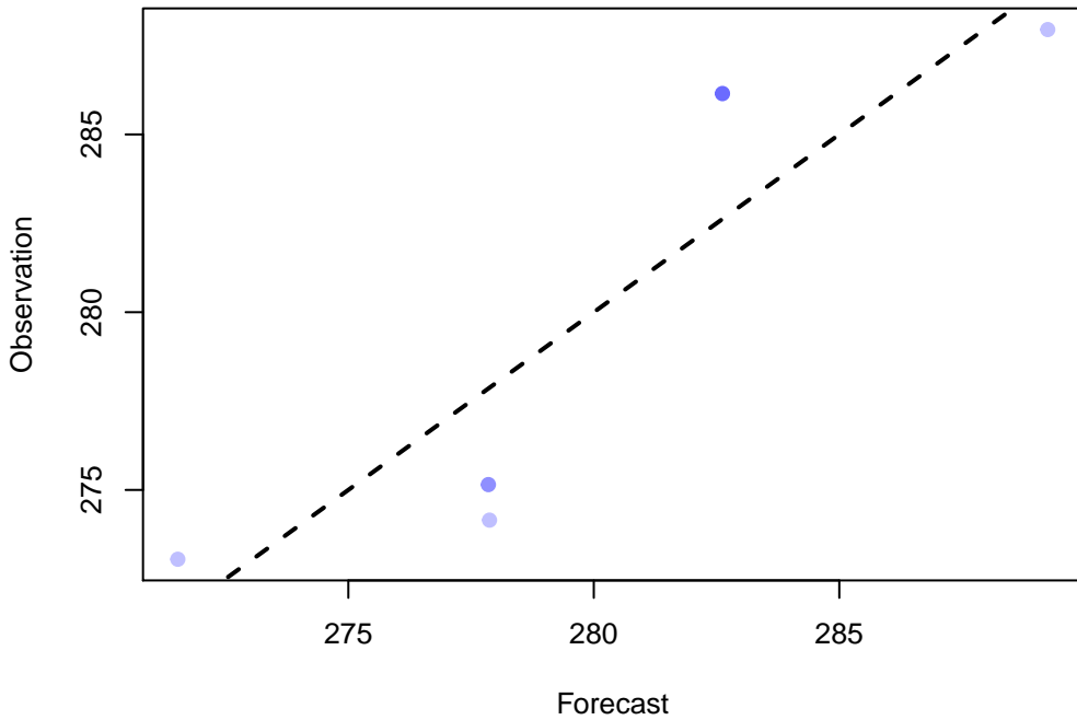
Scatter Plot of 8 points WRF: TMP at P900-750 ADPSFC, DTC166, MEDIAN(9)
