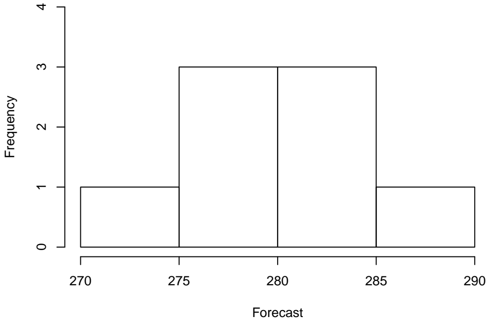
Forecast Histogram of 8 points WRF: TMP at P900-750 ADPSFC, DTC166, DW_MEAN(9)
