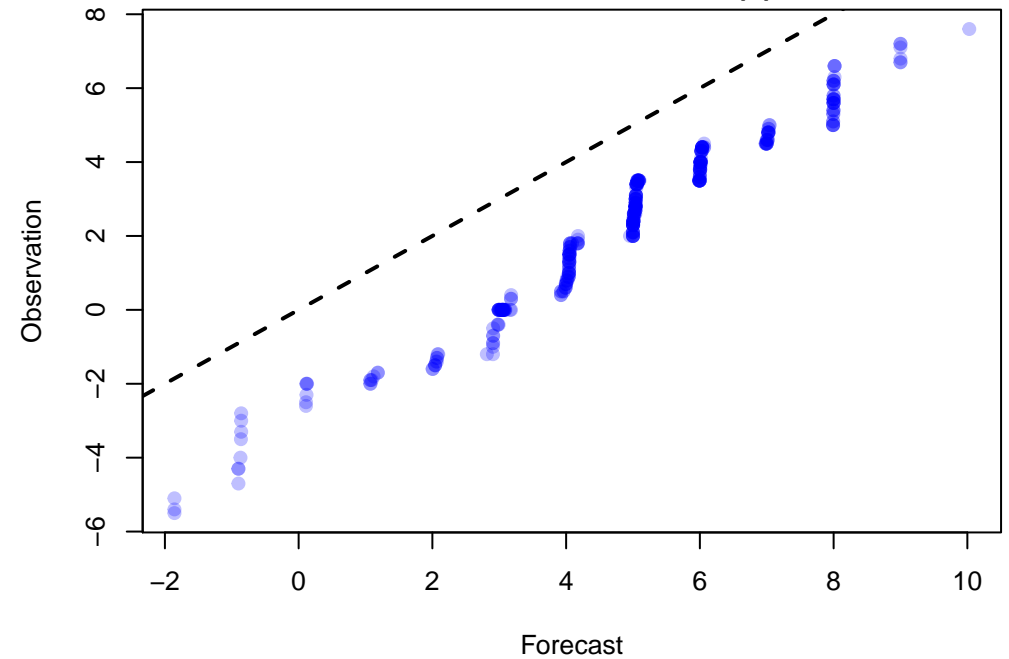
Q-Q Plot of 362 points WRF: VGRD at Z10 ADPSFC, LMV, MEDIAN(9)
