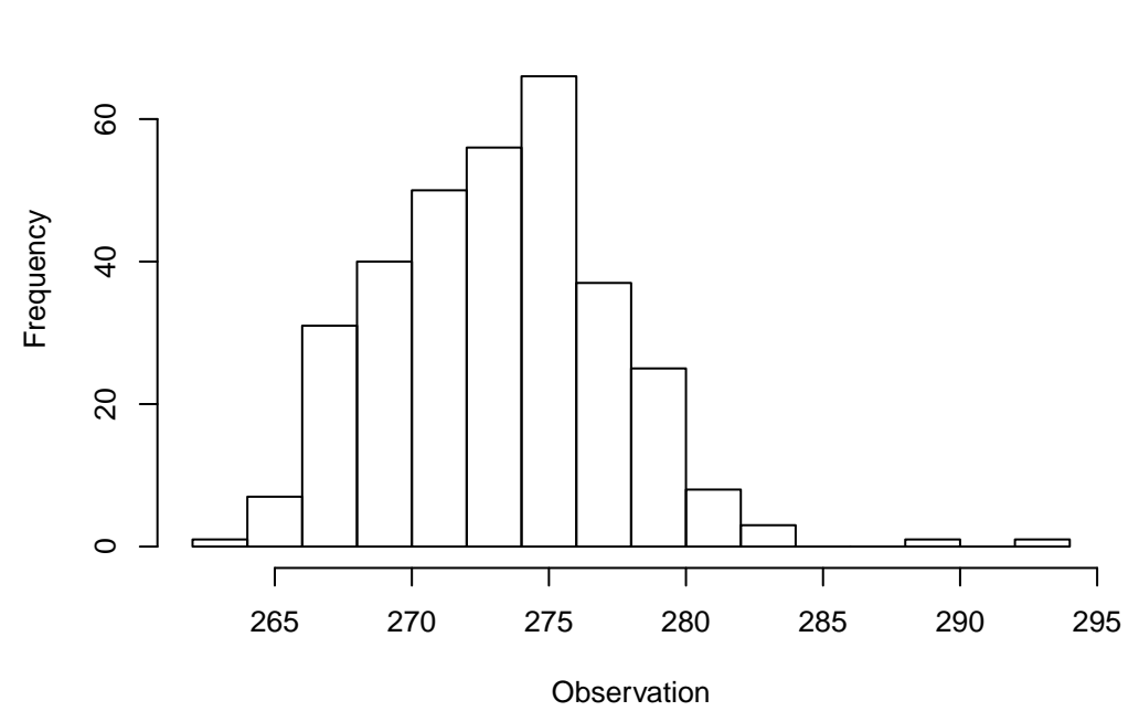
Observation Histogram of 326 points WRF: TMP at P900-750 ADPSFC, DTC165, DW_MEAN(9)
