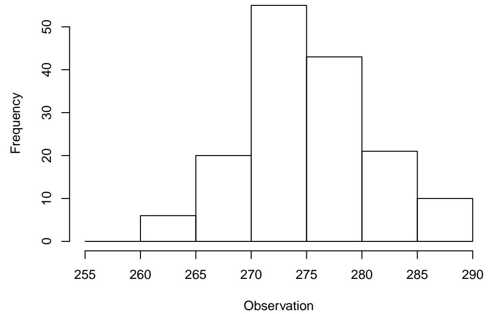
Observation Histogram of 155 points WRF: TMP at P900-750 ADPUPA, DTC165, DW_MEAN(9)
