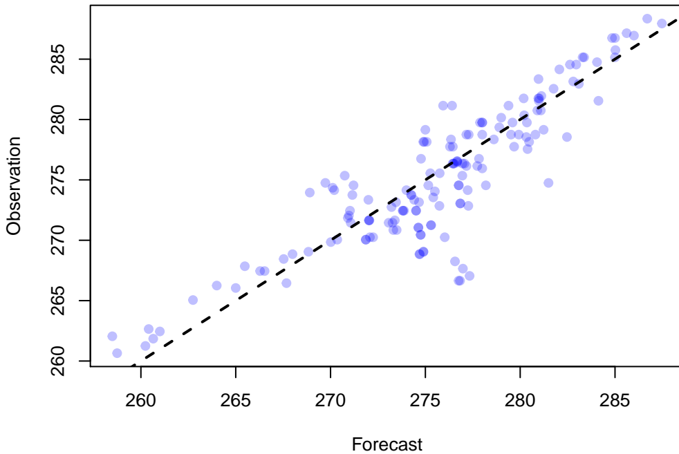
Scatter Plot of 155 points WRF: TMP at P900-750 ADPUPA, DTC165, DW_MEAN(9)
