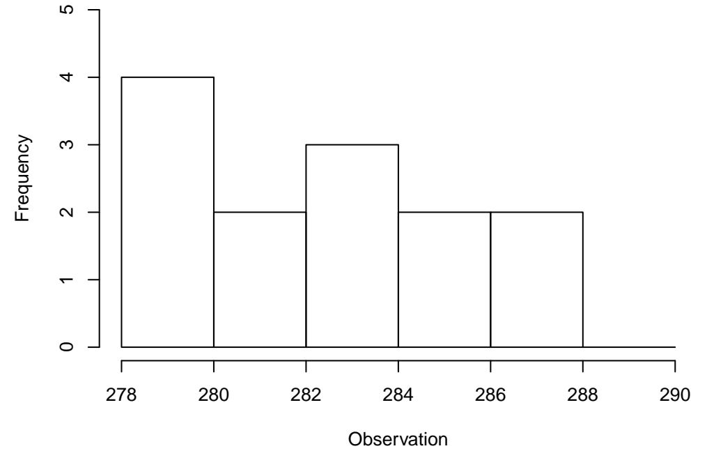
Observation Histogram of 13 points WRF: TMP at P900-750 ADPUPA, LMV, MEDIAN(9)
