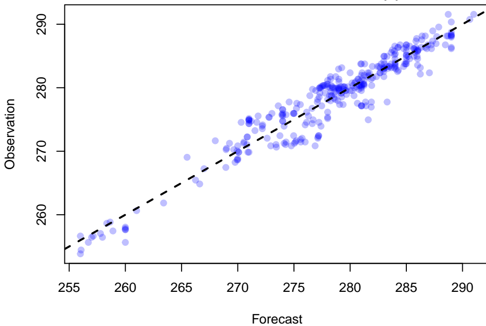
Scatter Plot of 334 points WRF: TMP at P900-750 ADPUPA, DTC166, UW_MEAN(1)
