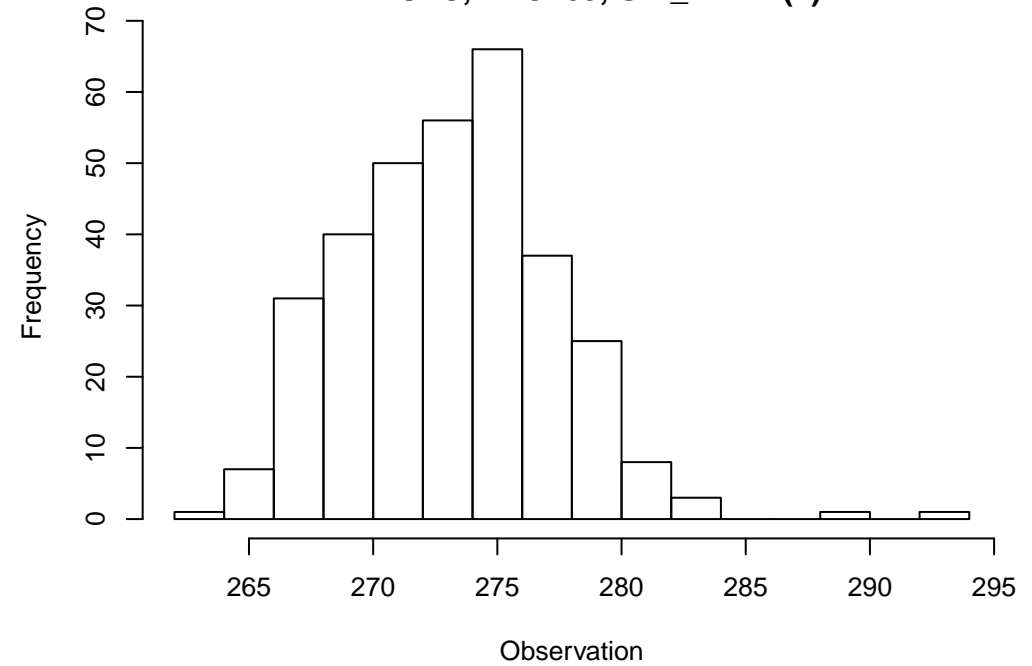
Observation Histogram of 326 points WRF: TMP at P900-750 ADPSFC, DTC165, UW_MEAN(1)
