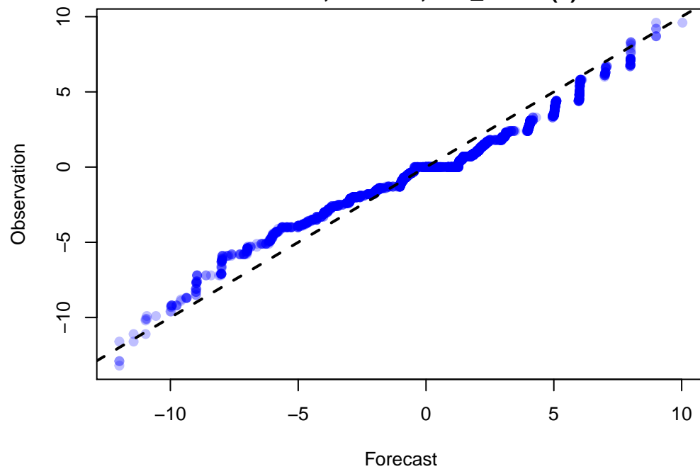
Q-Q Plot of 2955 points WRF: VGRD at Z10 ADPSFC, DTC166, UW_MEAN(1)
