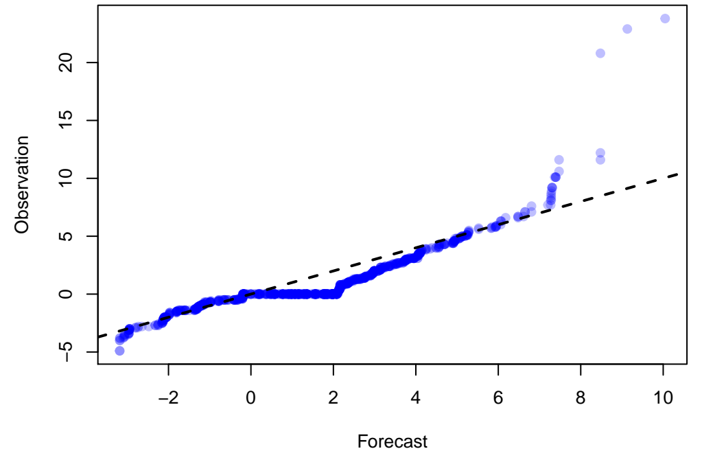
Q-Q Plot of 934 points WRF: UGRD at Z10 ADPSFC, DTC165, MEDIAN(9)
