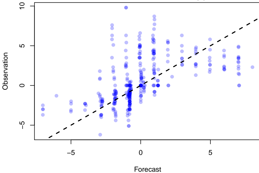
Scatter Plot of 362 points WRF: UGRD at Z10 ADPSFC, LMV, UW_MEAN(1)
