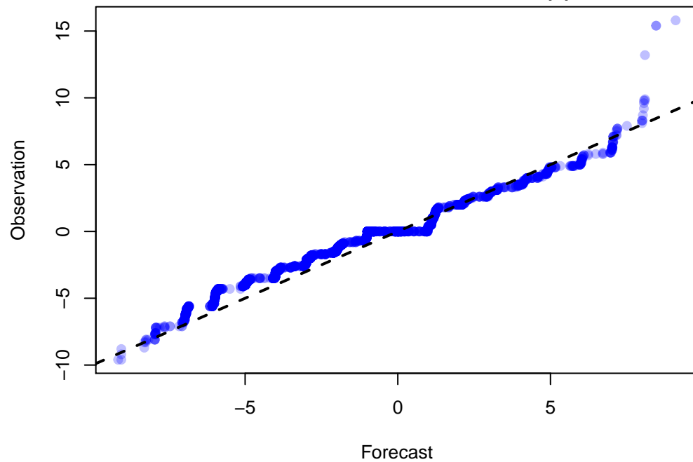
Q-Q Plot of 2955 points WRF: UGRD at Z10 ADPSFC, DTC166, UW_MEAN(1)
