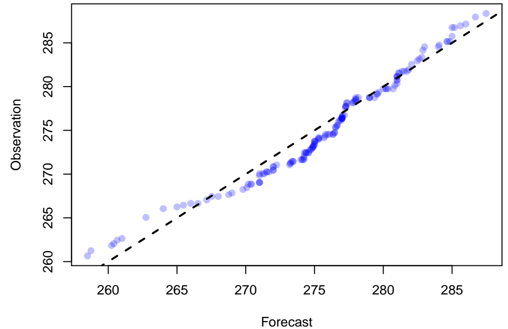
Q-Q Plot of 155 points WRF: TMP at P900-750 ADPUPA, DTC165, MEDIAN(9)
