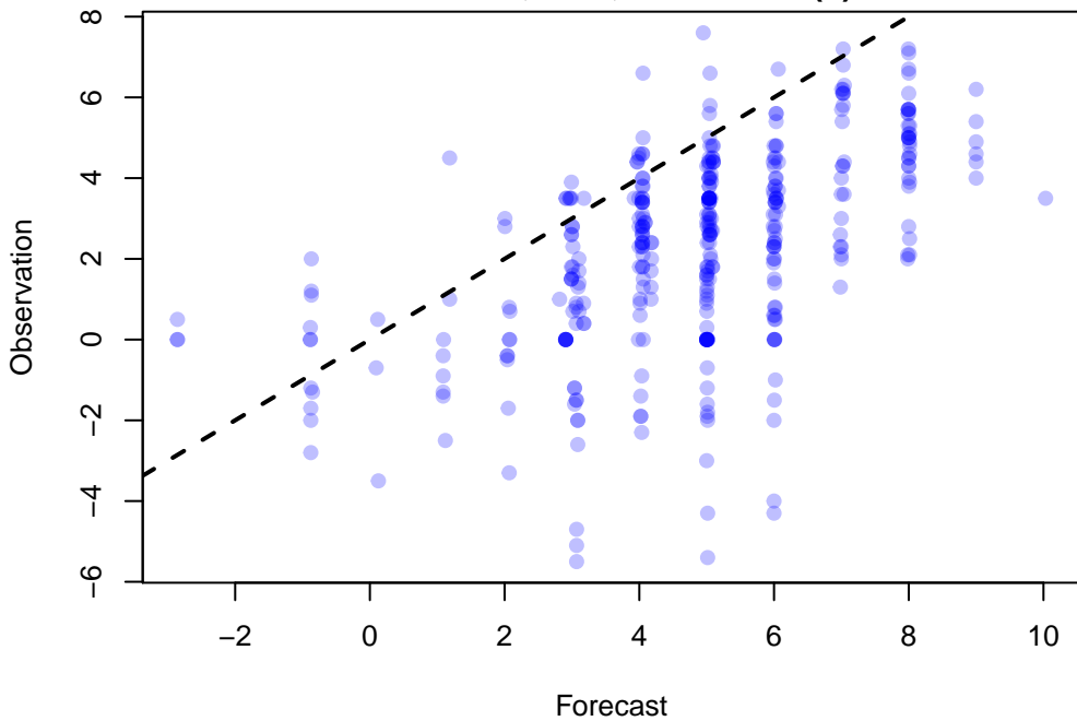
Scatter Plot of 362 points WRF: VGRD at Z10 ADPSFC, LMV, UW_MEAN(1)
