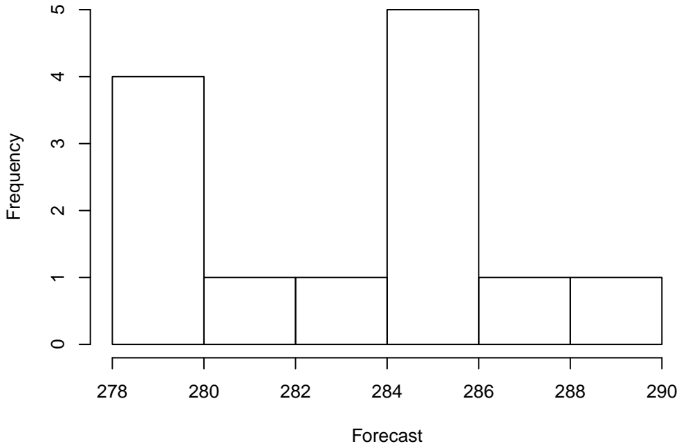
Forecast Histogram of 13 points WRF: TMP at P900-750 ADPUPA, LMV, UW_MEAN(1)
