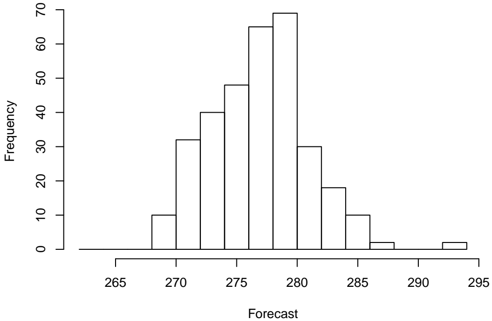
Forecast Histogram of 326 points WRF: TMP at P900-750 ADPSFC, DTC165, MEDIAN(9)
