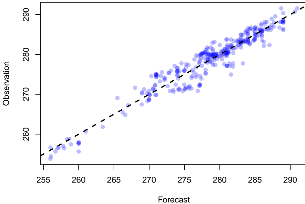
Scatter Plot of 334 points WRF: TMP at P900-750 ADPUPA, DTC166, MEDIAN(9)
