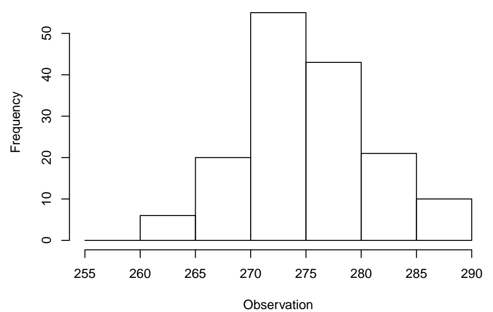
Observation Histogram of 155 points WRF: TMP at P900-750 ADPUPA, DTC165, MEDIAN(9)
