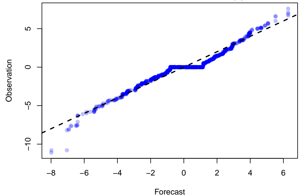
Q-Q Plot of 934 points WRF: VGRD at Z10 ADPSFC, DTC165, UW_MEAN(1)
