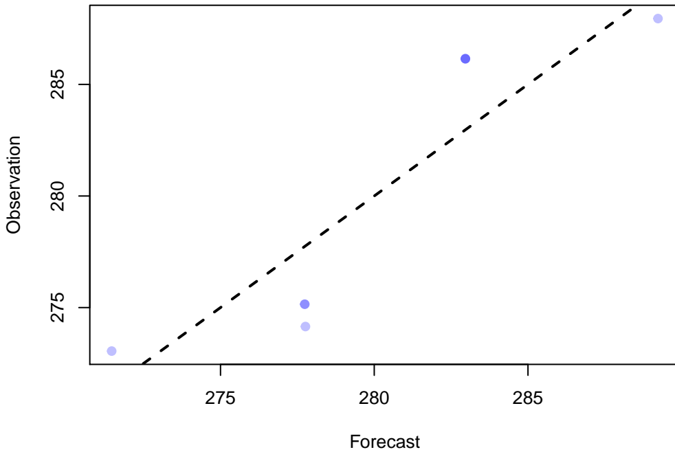
Scatter Plot of 8 points WRF: TMP at P900-750 ADPSFC, DTC166, DW_MEAN(9)
