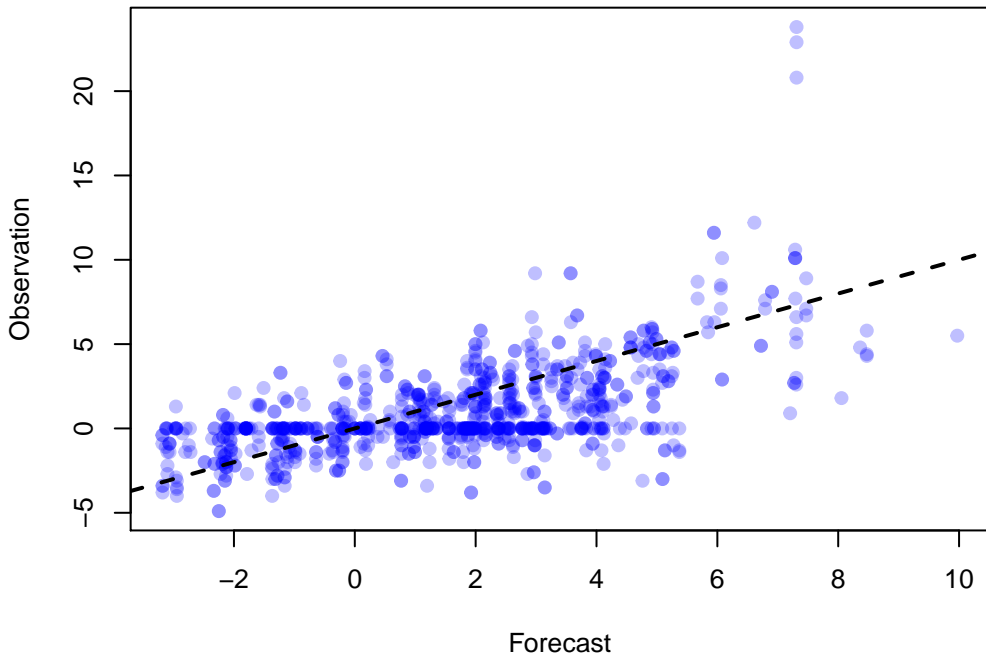
Scatter Plot of 934 points WRF: UGRD at Z10 ADPSFC, DTC165, UW_MEAN(1)
