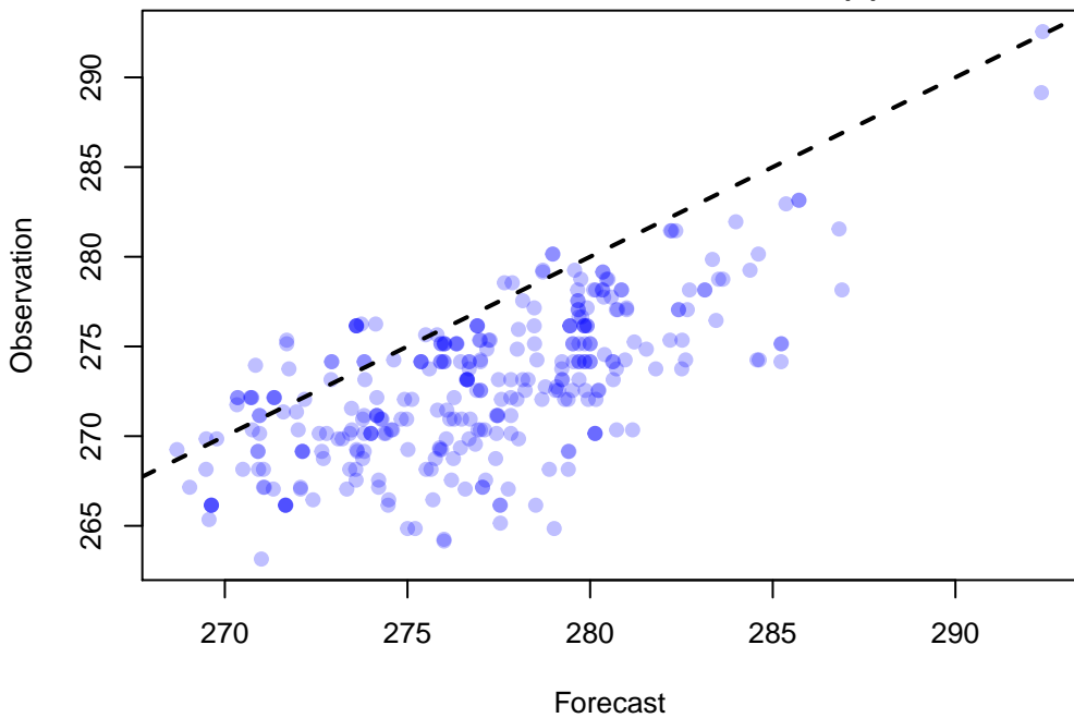
Scatter Plot of 326 points WRF: TMP at P900-750 ADPSFC, DTC165, UW_MEAN(1)
