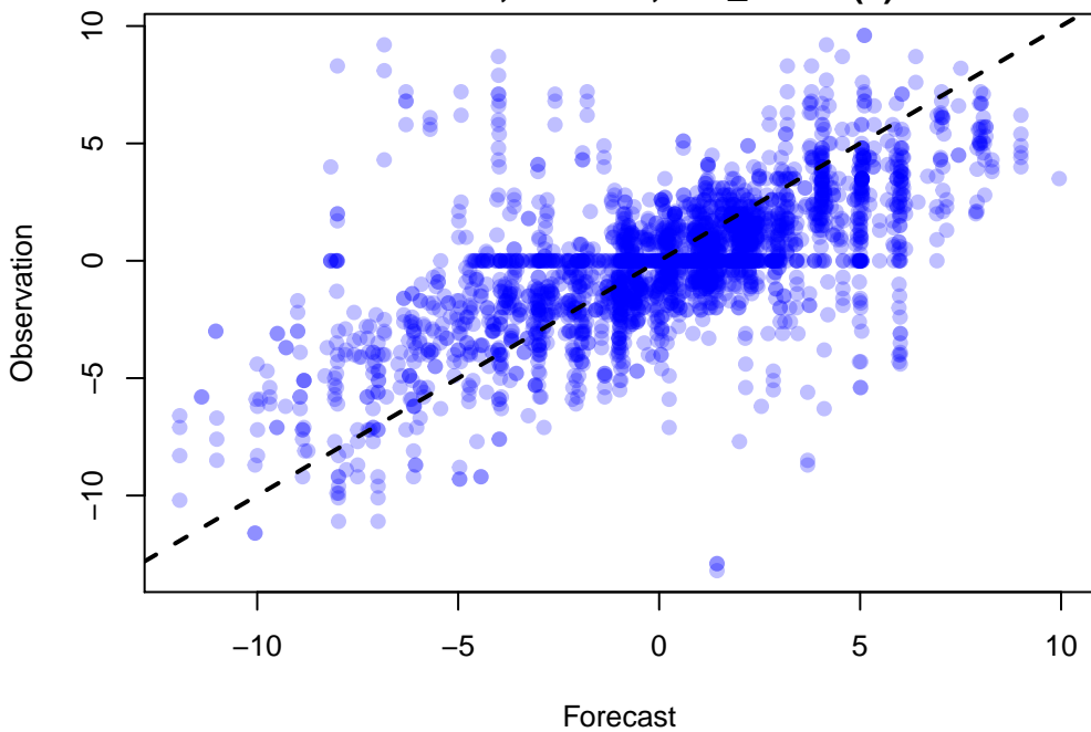
Scatter Plot of 2955 points WRF: VGRD at Z10 ADPSFC, DTC166, DW_MEAN(9)
