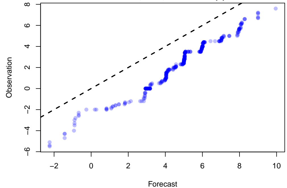
Q-Q Plot of 362 points WRF: VGRD at Z10 ADPSFC, LMV, DW_MEAN(9)
