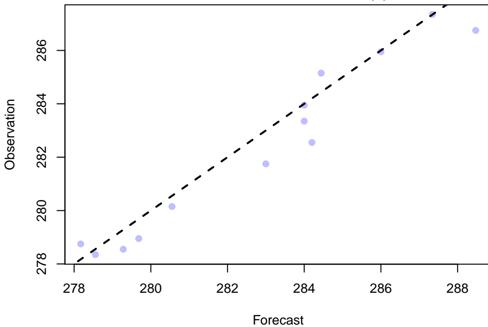
Scatter Plot of 13 points WRF: TMP at P900-750 ADPUPA, LMV, DW_MEAN(9)
