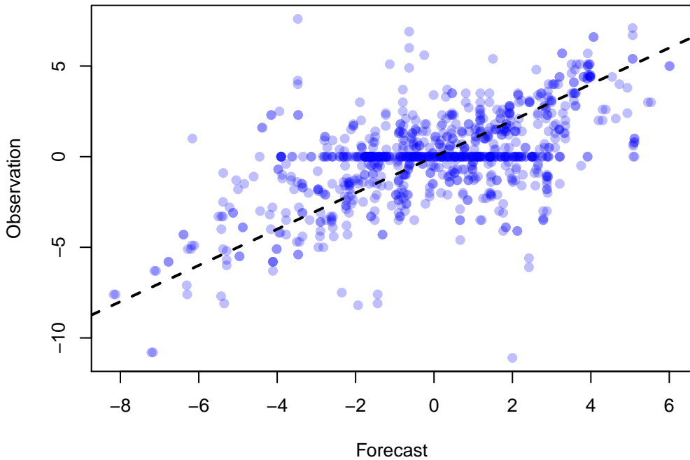
Scatter Plot of 934 points WRF: VGRD at Z10 ADPSFC, DTC165, DW_MEAN(9)
