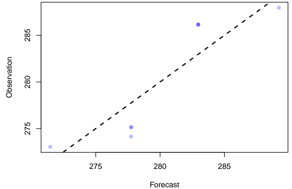
Q-Q Plot of 8 points WRF: TMP at P900-750 ADPSFC, DTC166, DW_MEAN(9)
