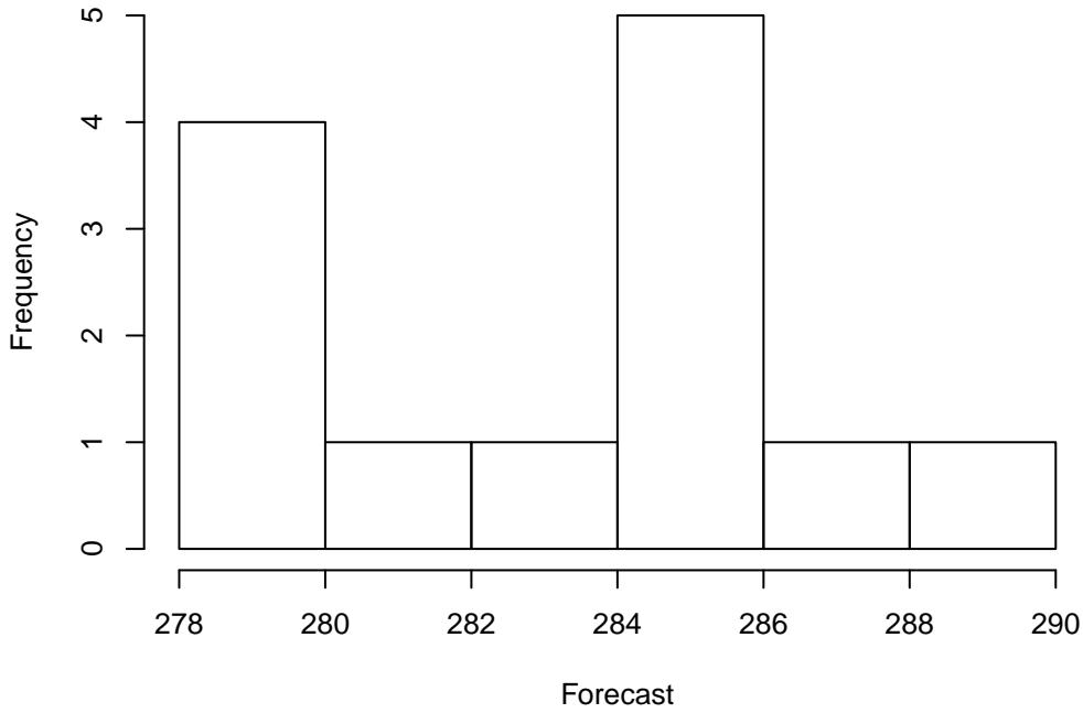
Forecast Histogram of 13 points WRF: TMP at P900-750 ADPUPA, LMV, MEDIAN(9)
