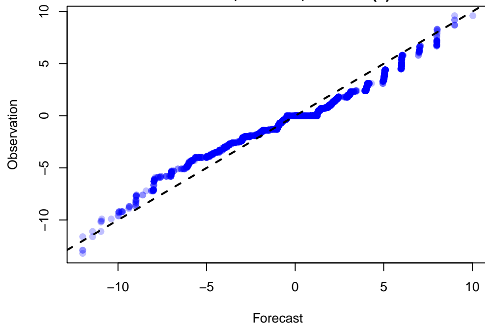
Q-Q Plot of 2955 points WRF: VGRD at Z10 ADPSFC, DTC166, MEDIAN(9)
