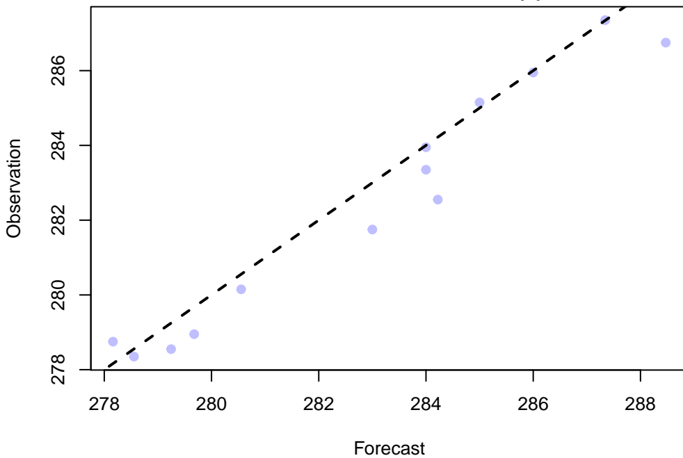
Scatter Plot of 13 points WRF: TMP at P900-750 ADPUPA, LMV, UW_MEAN(1)
