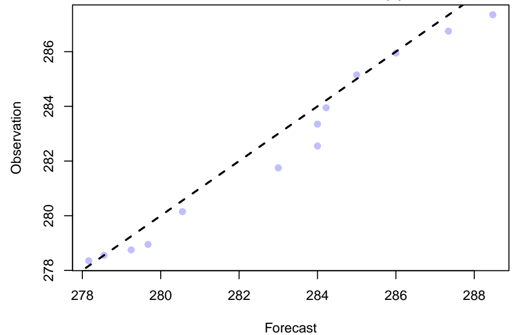
Q-Q Plot of 13 points WRF: TMP at P900-750 ADPUPA, LMV, UW_MEAN(1)
