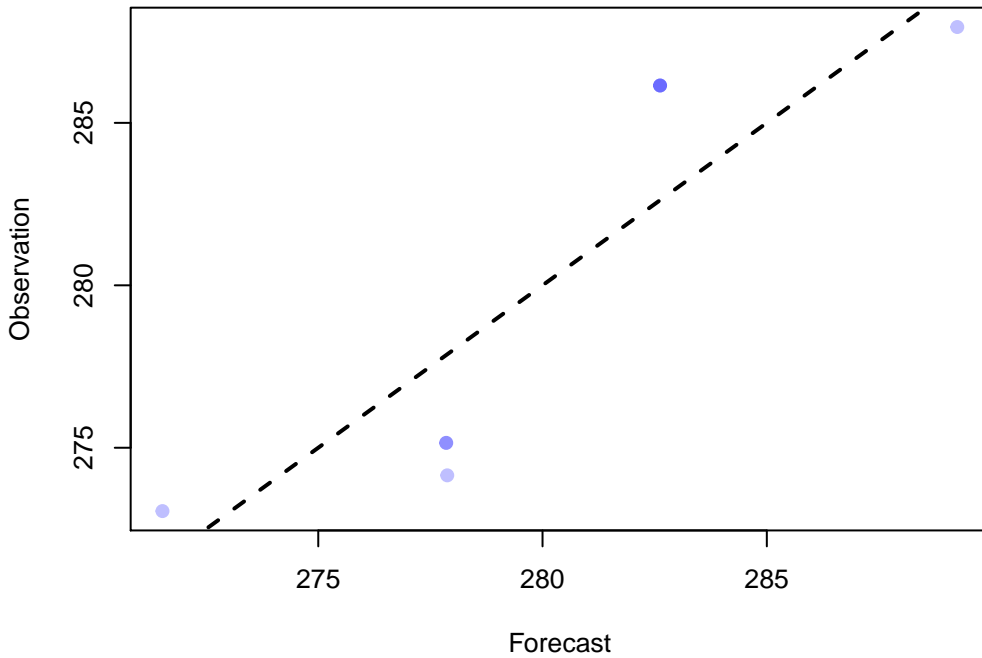
Scatter Plot of 8 points WRF: TMP at P900-750 ADPSFC, DTC166, UW_MEAN(1)
