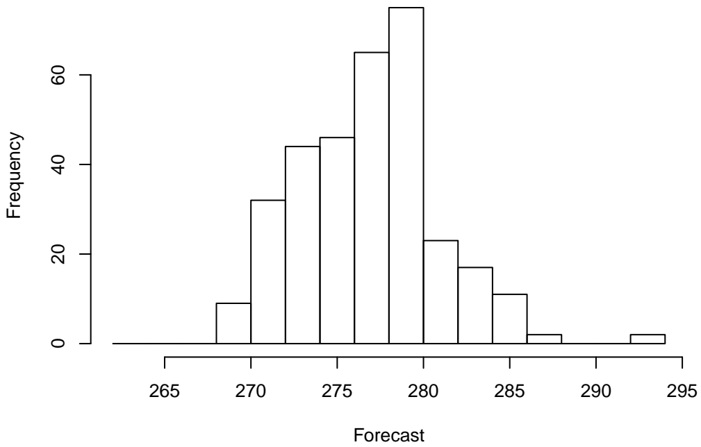
Forecast Histogram of 326 points WRF: TMP at P900-750 ADPSFC, DTC165, DW_MEAN(9)
