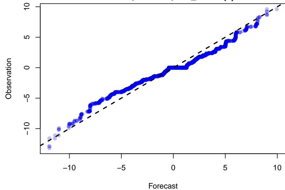
Q-Q Plot of 2955 points WRF: VGRD at Z10 ADPSFC, DTC166, DW_MEAN(9)
