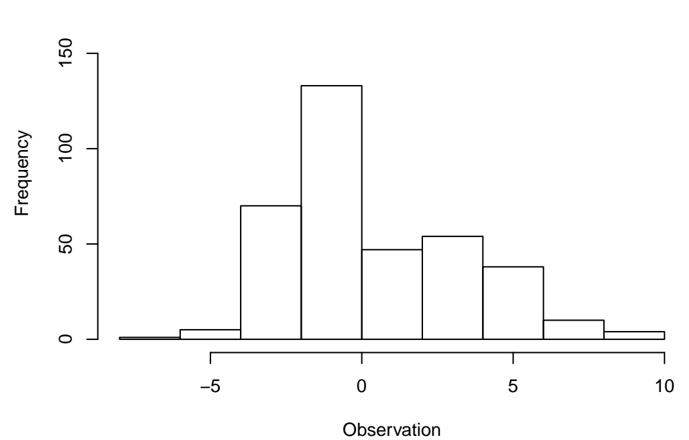
Observation Histogram of 362 points WRF: UGRD at Z10 ADPSFC, LMV, UW_MEAN(1)
