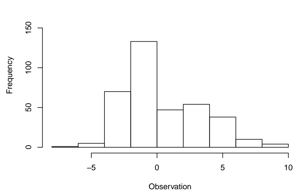
Observation Histogram of 362 points WRF: UGRD at Z10 ADPSFC, LMV, DW_MEAN(9)
