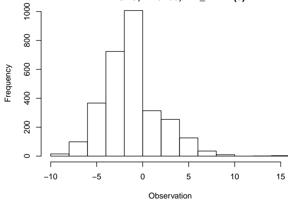
Observation Histogram of 2955 points WRF: UGRD at Z10 ADPSFC, DTC166, DW_MEAN(9)
