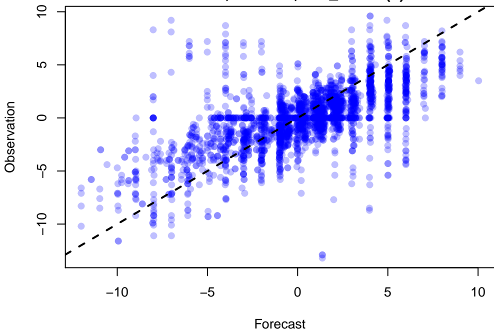
Scatter Plot of 2955 points WRF: VGRD at Z10 ADPSFC, DTC166, UW_MEAN(1)
