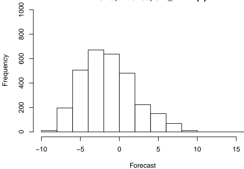
Forecast Histogram of 2955 points WRF: UGRD at Z10 ADPSFC, DTC166, UW_MEAN(1)
