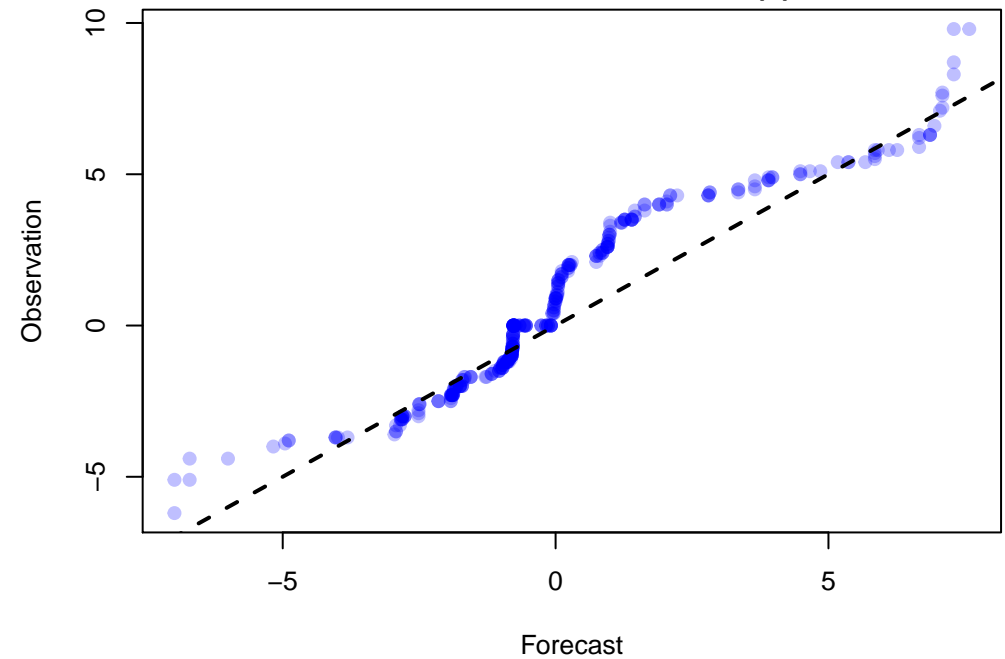
Q-Q Plot of 362 points WRF: UGRD at Z10 ADPSFC, LMV, DW_MEAN(9)
