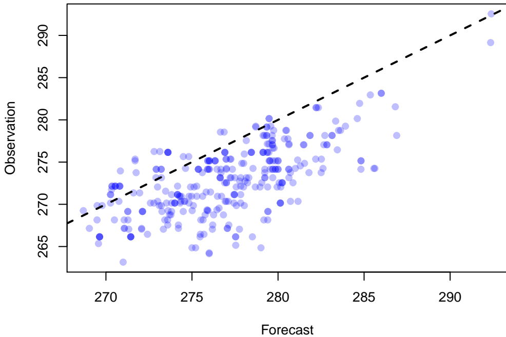
Scatter Plot of 326 points WRF: TMP at P900-750 ADPSFC, DTC165, MEDIAN(9)
