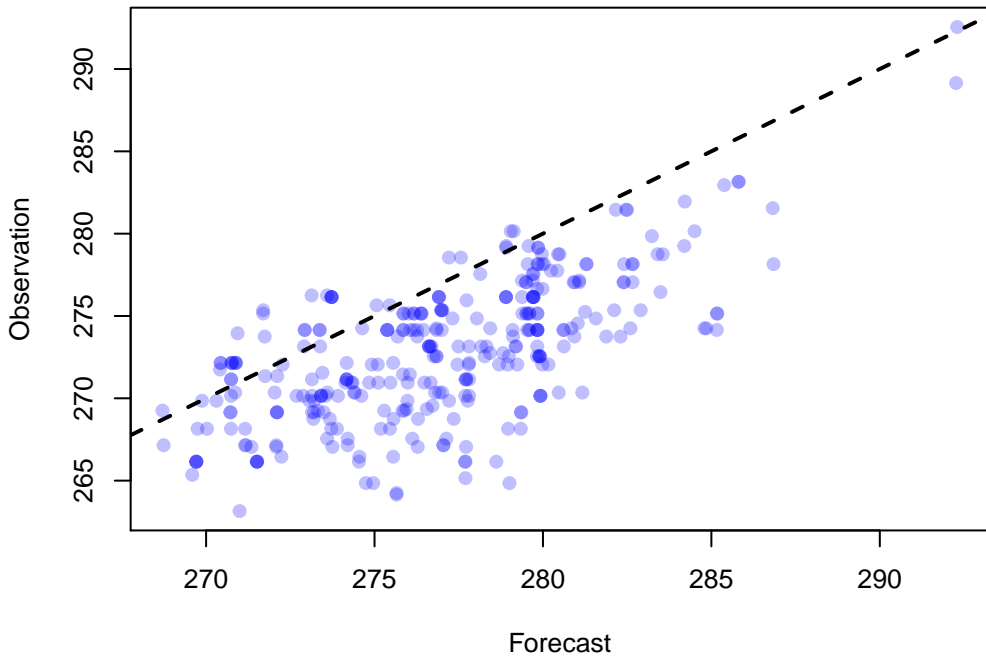
Scatter Plot of 326 points WRF: TMP at P900-750 ADPSFC, DTC165, DW_MEAN(9)
