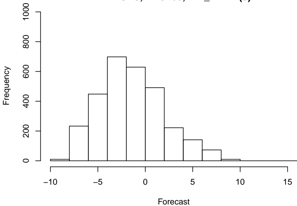
Forecast Histogram of 2955 points WRF: UGRD at Z10 ADPSFC, DTC166, DW_MEAN(9)
