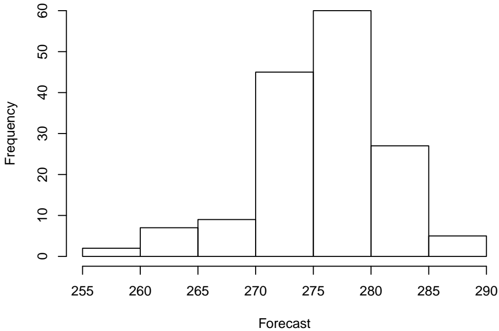
Forecast Histogram of 155 points WRF: TMP at P900-750 ADPUPA, DTC165, UW_MEAN(1)
