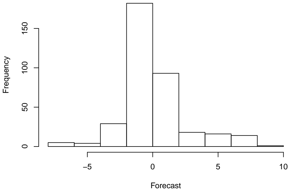
Forecast Histogram of 362 points WRF: UGRD at Z10 ADPSFC, LMV, MEDIAN(9)
