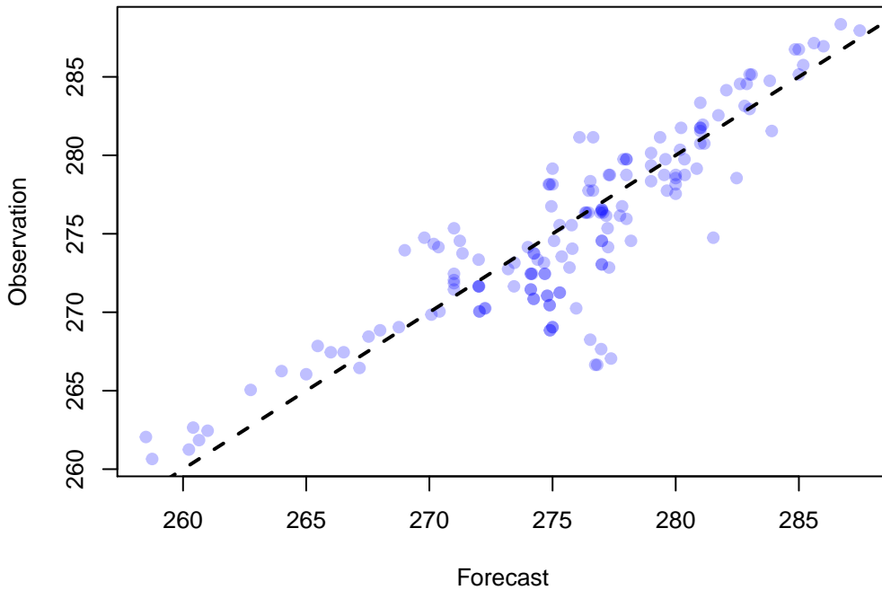
Scatter Plot of 155 points WRF: TMP at P900-750 ADPUPA, DTC165, UW_MEAN(1)
