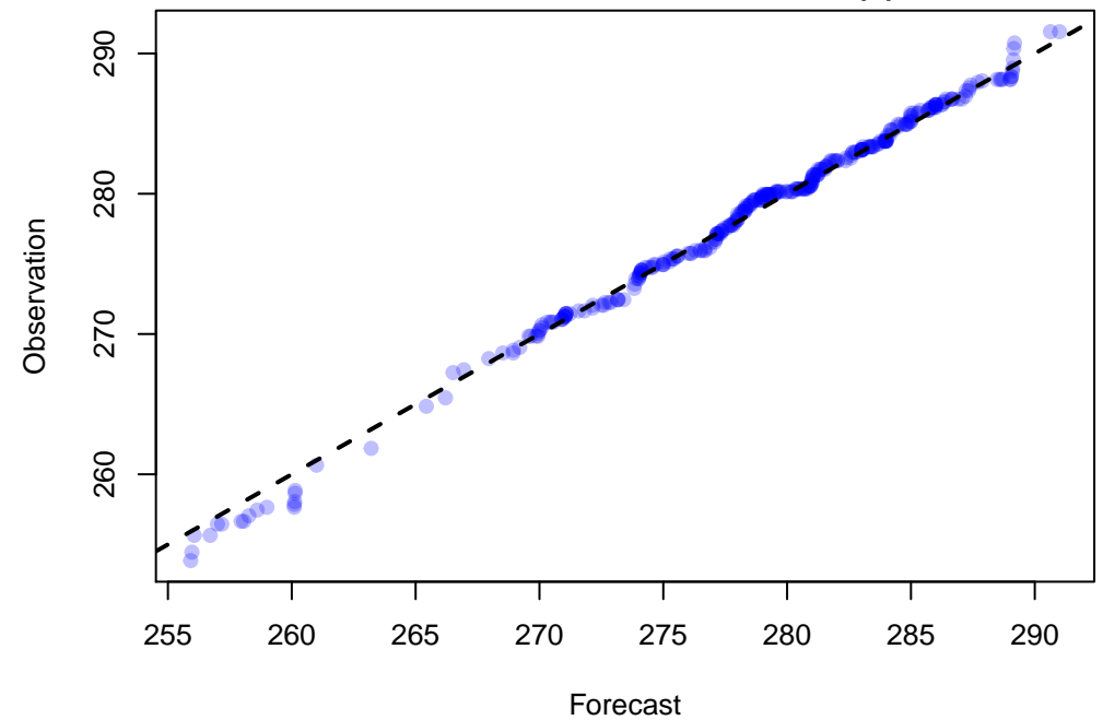
Q-Q Plot of 334 points WRF: TMP at P900-750 ADPUPA, DTC166, DW_MEAN(9)
