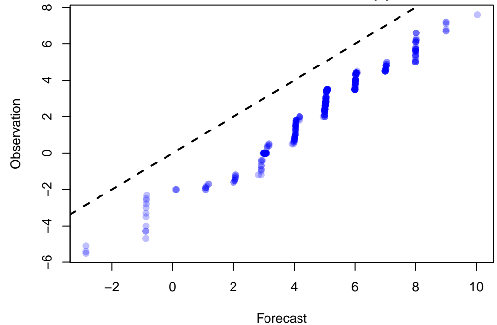
Q-Q Plot of 362 points WRF: VGRD at Z10 ADPSFC, LMV, UW_MEAN(1)
