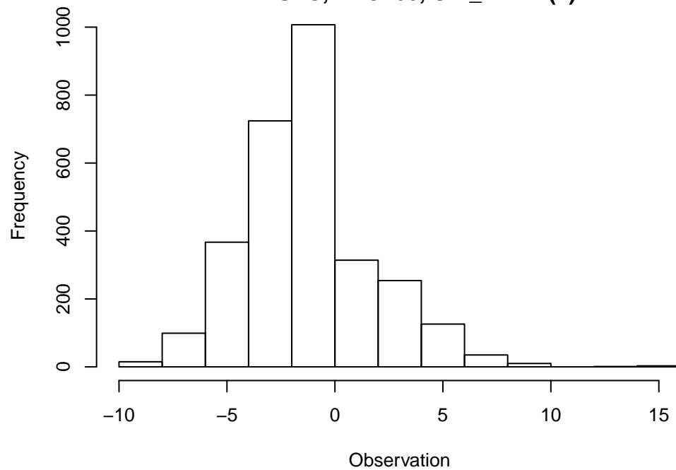
Observation Histogram of 2955 points WRF: UGRD at Z10 ADPSFC, DTC166, UW_MEAN(1)
