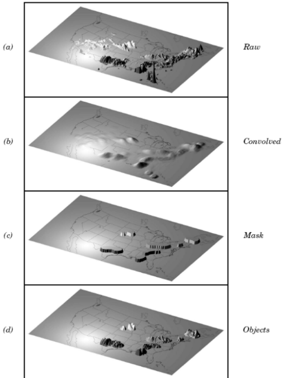
Figure 14.1: Example of an application of the MODO object identification process to a model precipitation field.
