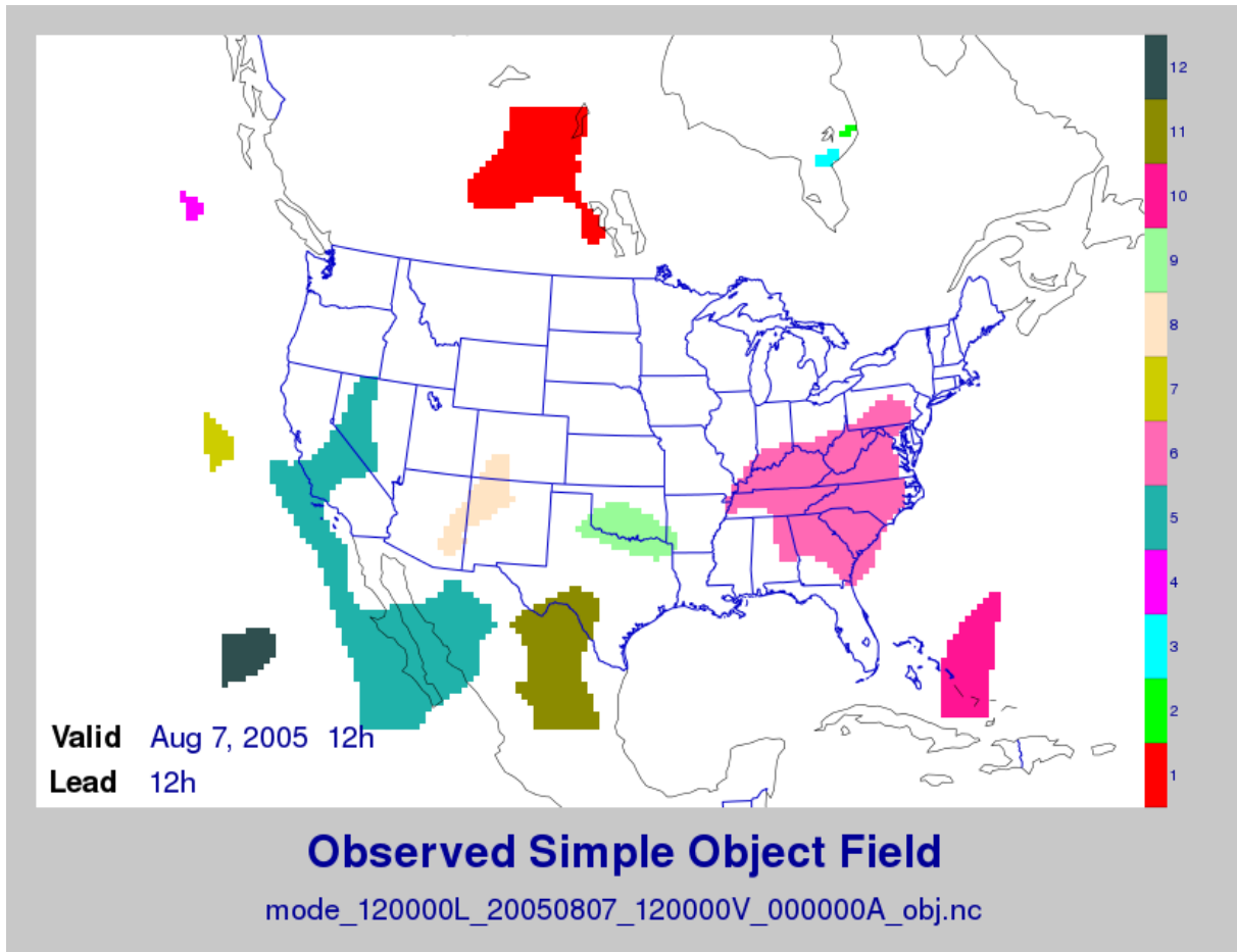
Figure 21.1: Simple observed precipitation objects
