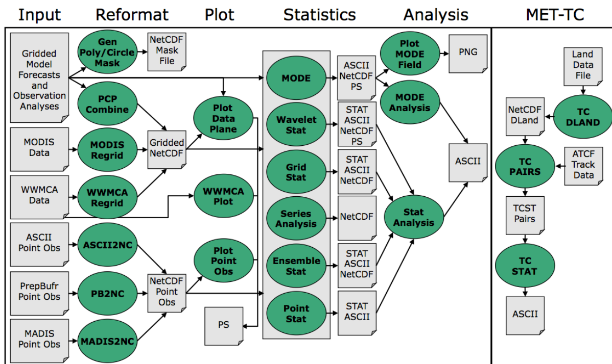
Figure 1-0-1. Basic representation of current MET structure and modules. Colored areas represent software and modules included in MET, and gray areas represent input and output files.
