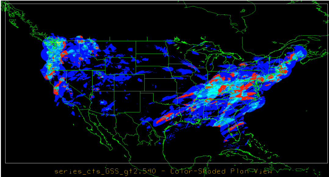
Figure 6-1: An example of the Gilbert Skill Score for precipitation forecasts at each grid location for a month of files.
