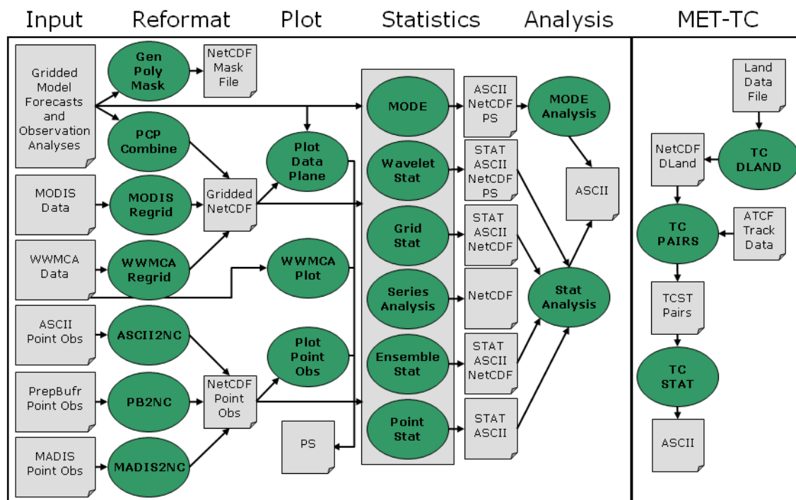
Figure 1-0-1. Basic representation of current MET structure and modules. Green areas represent software and modules included in MET, and gray areas represent input and output files.
