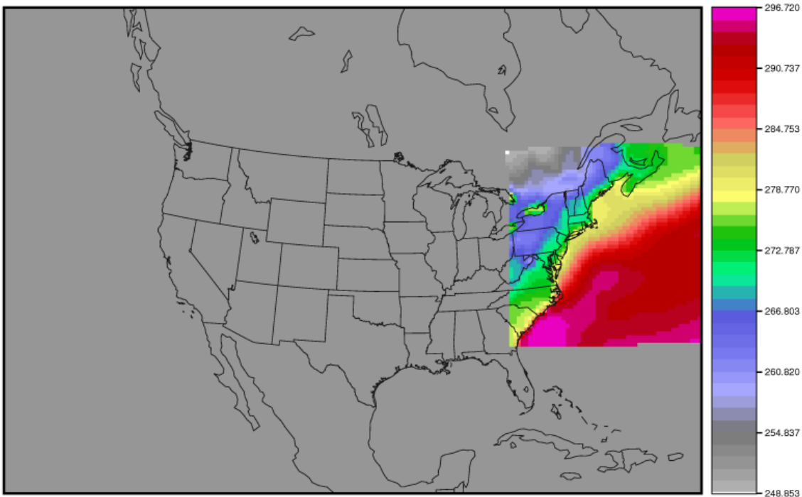
Figure 3-1: Example plot showing surface temperature from a MODIS file.
