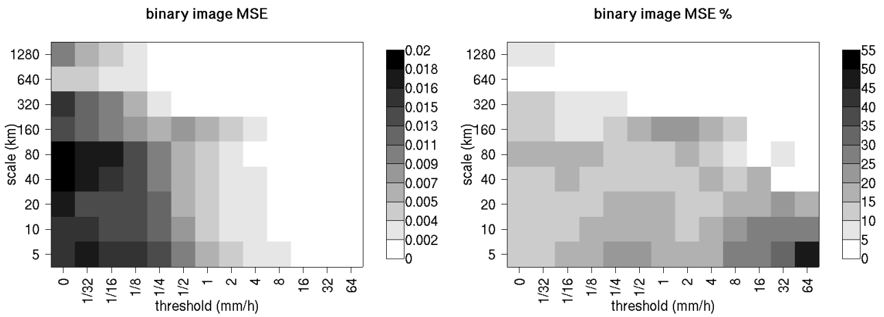
Figure 9.4: MSE and MSE % for the NIMROD binary forecast and analysis spatial scale components. In the MSE%, note the large error associated to the scale 6 = 160 km, for the thresholds \frac{1}{2} to 4 mm/h, associated to the displaced storm.
