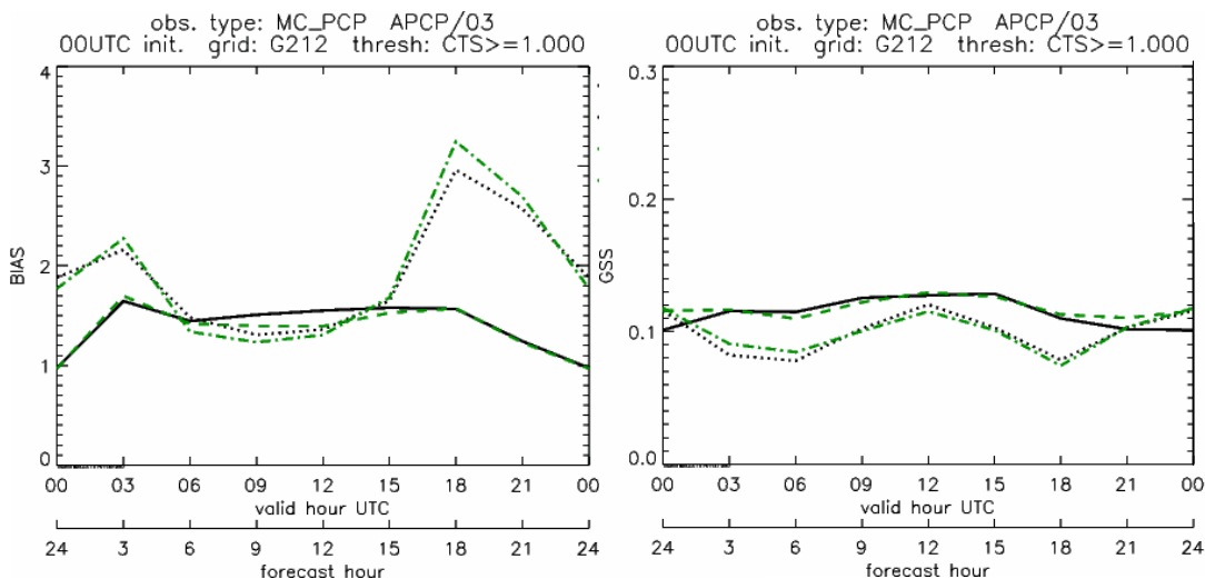
Figure 12-1: Time series of forecast area bias and Gilbert Skill Score for four model configurations (different lines) stratified by time-of-day.
