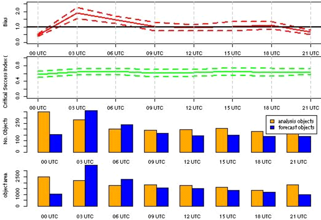
Figure 12-2: Traditional verification scores applied to output of the MODE tool, computed by defining matched observed objects to be hits, unmatched observed objects to be misses, and unmatched forecast objects to be false alarms; weighted by object area. Bar plots show numbers (penultimate row) and areas (bottom row) of observed and forecast objects, respectively.
