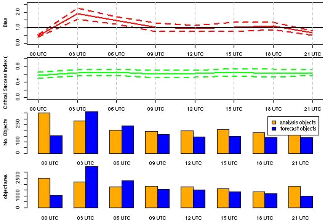
Figure 11-2: Traditional verification scores applied to output of the MODE tool, computed by defining matched observed objects to be hits, unmatched observed objects to be misses, and unmatched forecast objects to be false alarms; weighted by object area. Bar plots show numbers (penultimate row) and areas (bottom row) of observed and forecast objects, respectively.
