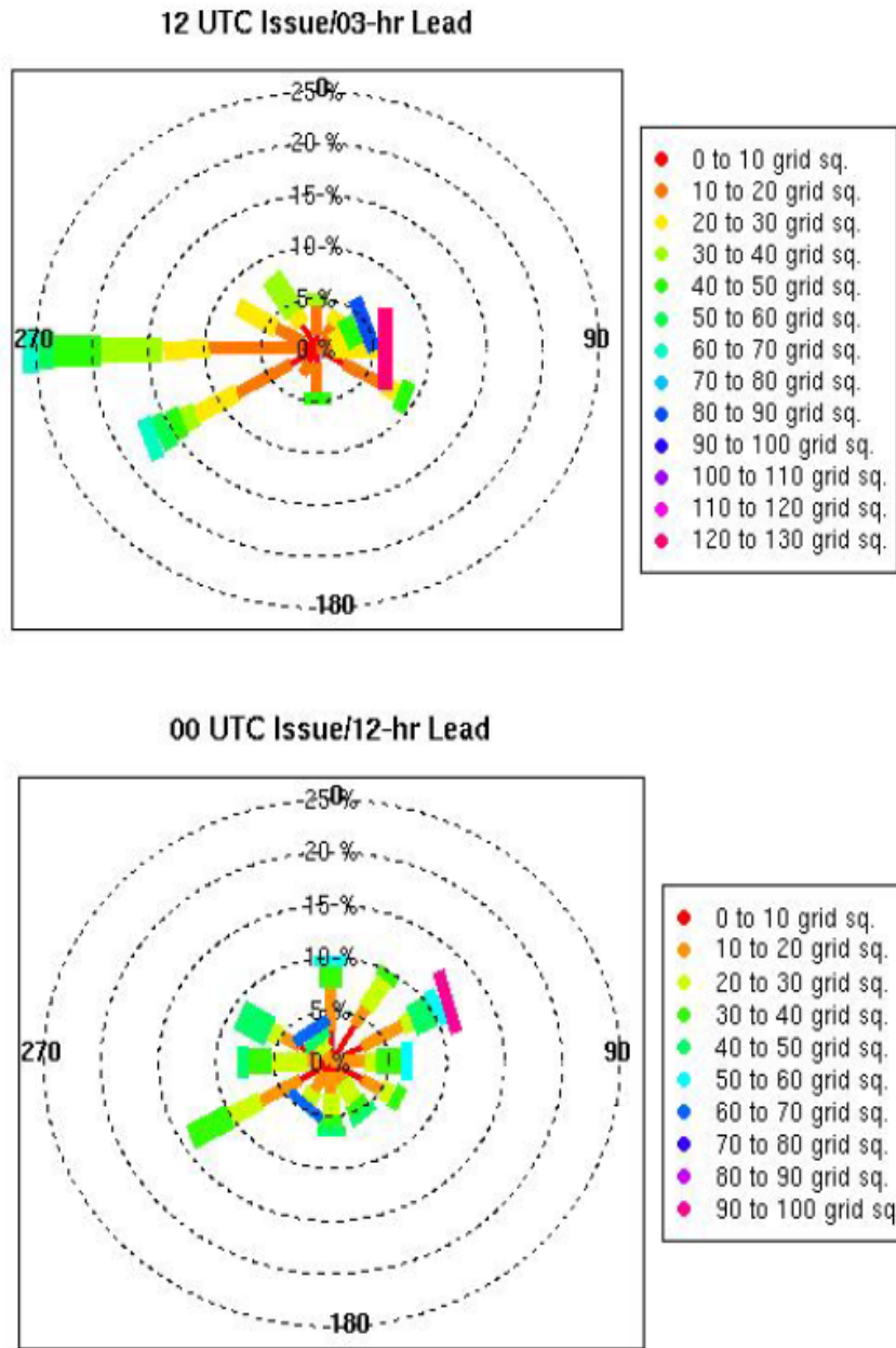
Figure 11-3: Circle histograms showing object centroid angles and distances (see text for explanation).
