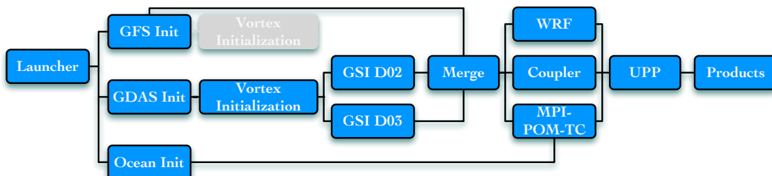
Figure 3.1: Components of HWRP that run for the default AL and EP configuration.
