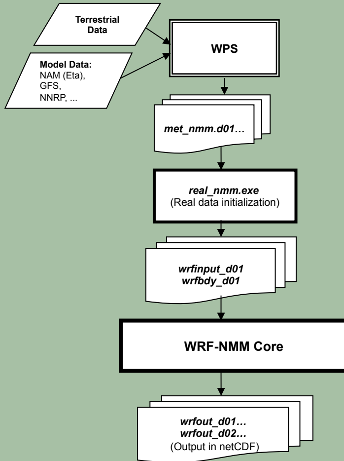
WRF-NMM FLOW CHART
