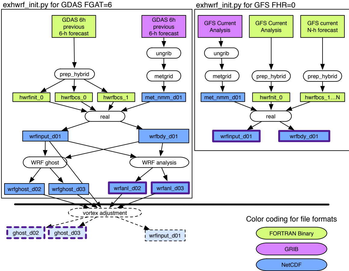
Figure 4.3: Simplified initialization procedures for the HWRF analysis time. All processes in the black box on the left are run by calling exhwrp_init.py for GDAS at FGAT=6, while those in the black box on the right are procedures run by calling exhwrp_init.py for GFS at the analysis time. Colored rectangles indicate input and output files, while white ovals are executable programs. Boxes with dashed outlines indicate modules and resulting files that are discussed in Chapter 5. Files that are outlined in heavy purple (dashed or solid) are used by subsequent processes described by Figure 6.1.
