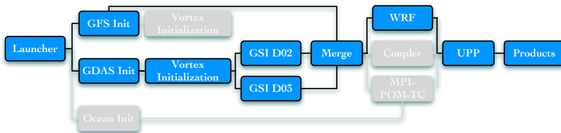
Figure 3.4: Components of HWRF that run for the uncoupled configuration.
